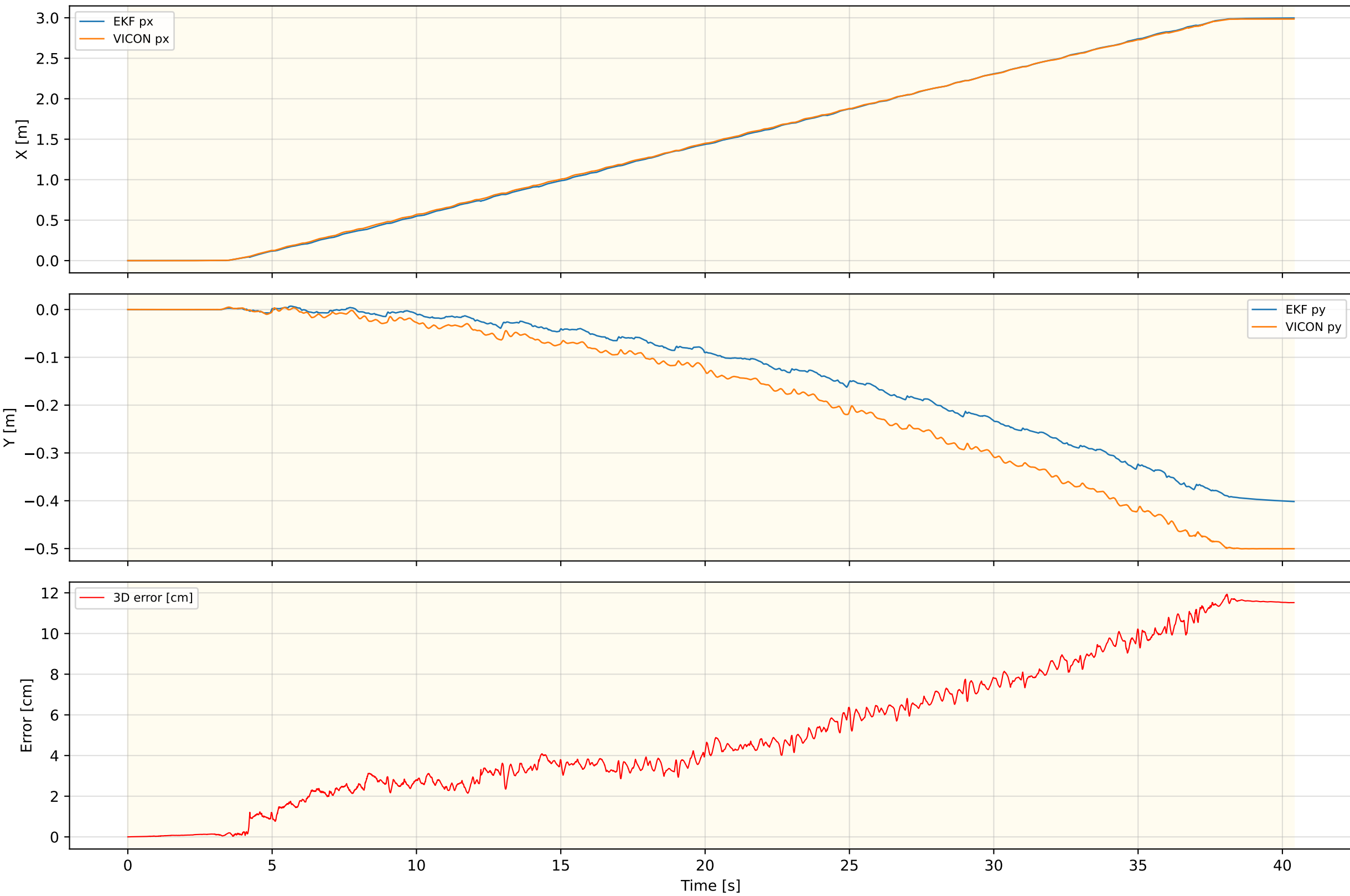
Inner EKF Position — FLAT_MPC_NEW_REAL_1
