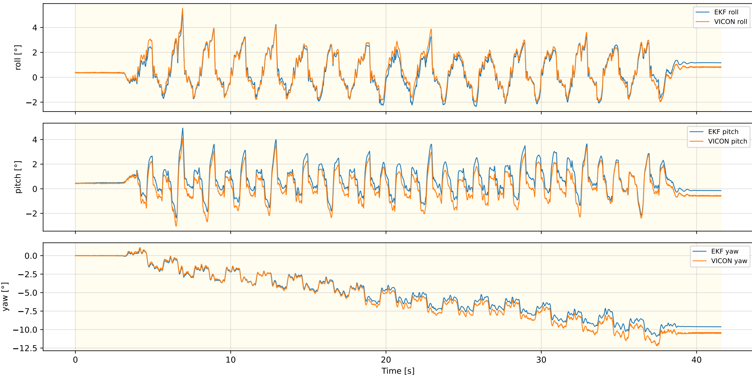
Inner EKF Attitude — FLAT_MPC_NEW_REAL_2
