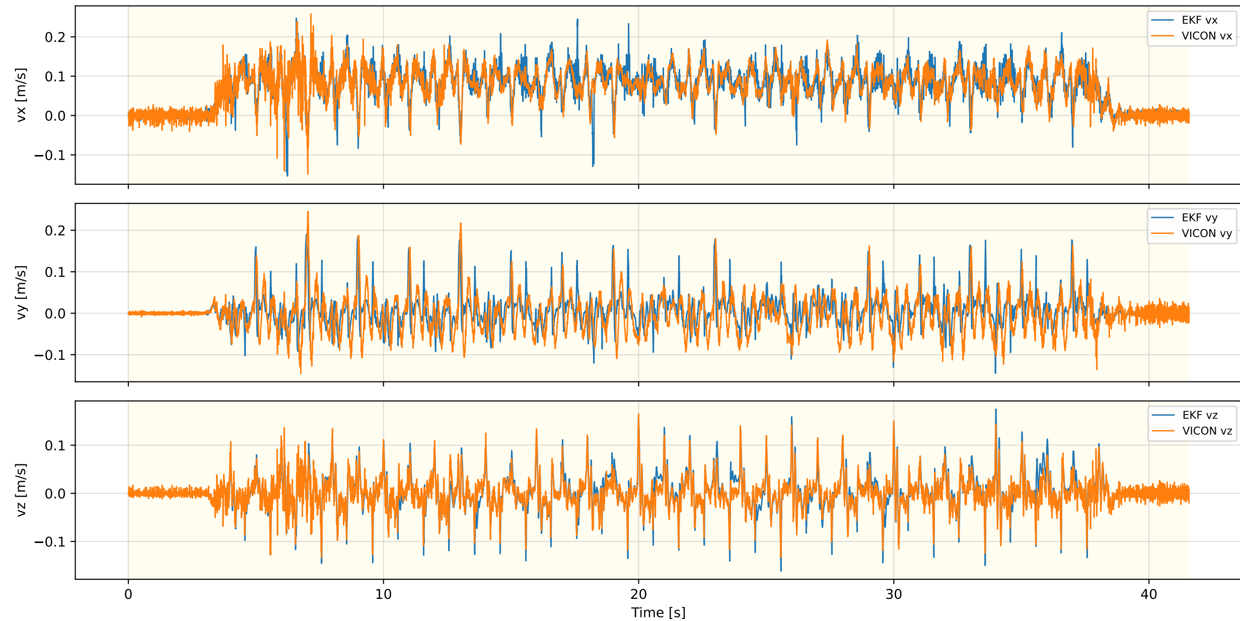
Inner EKF Velocity — FLAT_MPC_NEW_REAL_2
