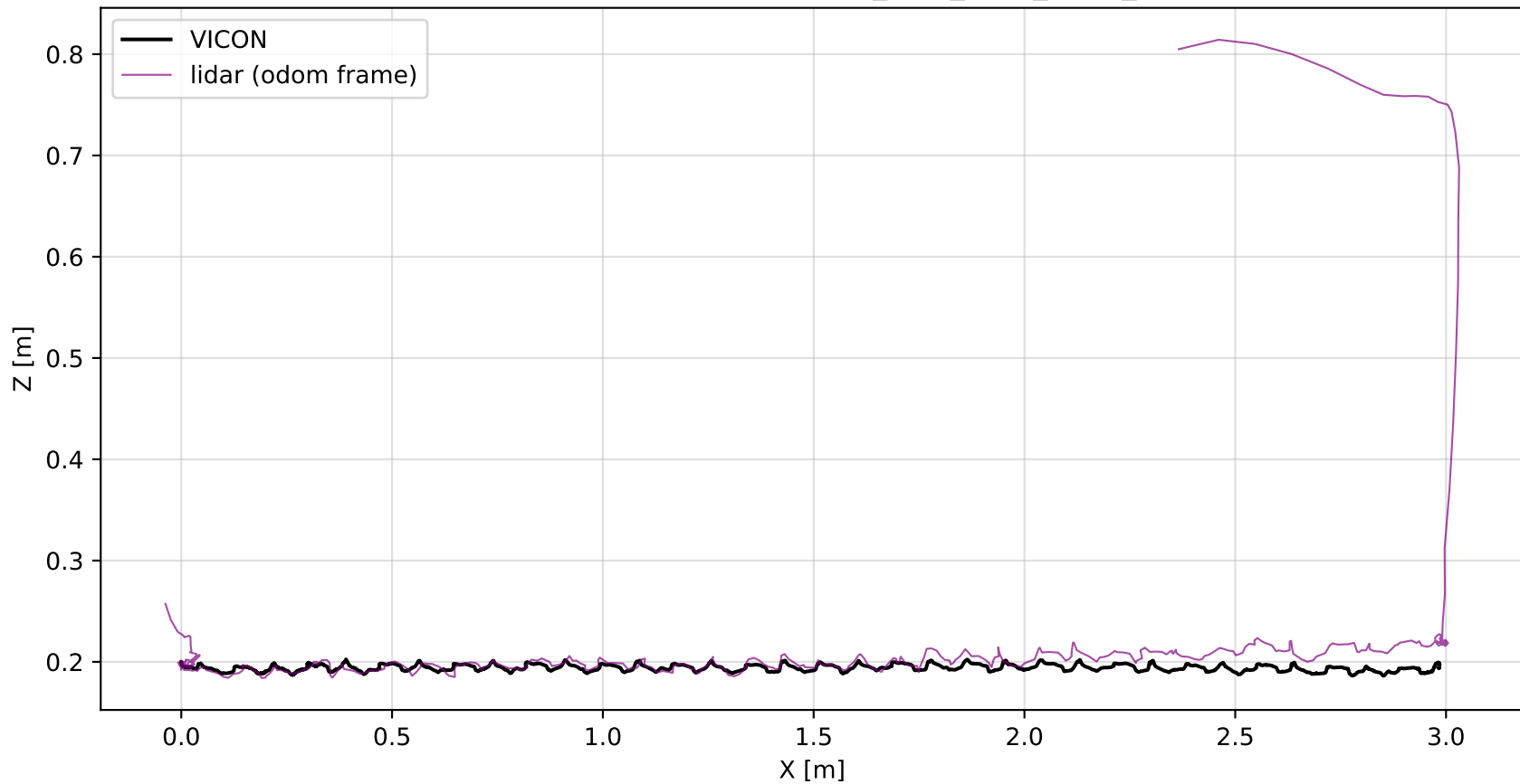
LiDAR XZ Trajectory — FLAT_MPC_NEW_REAL_2
