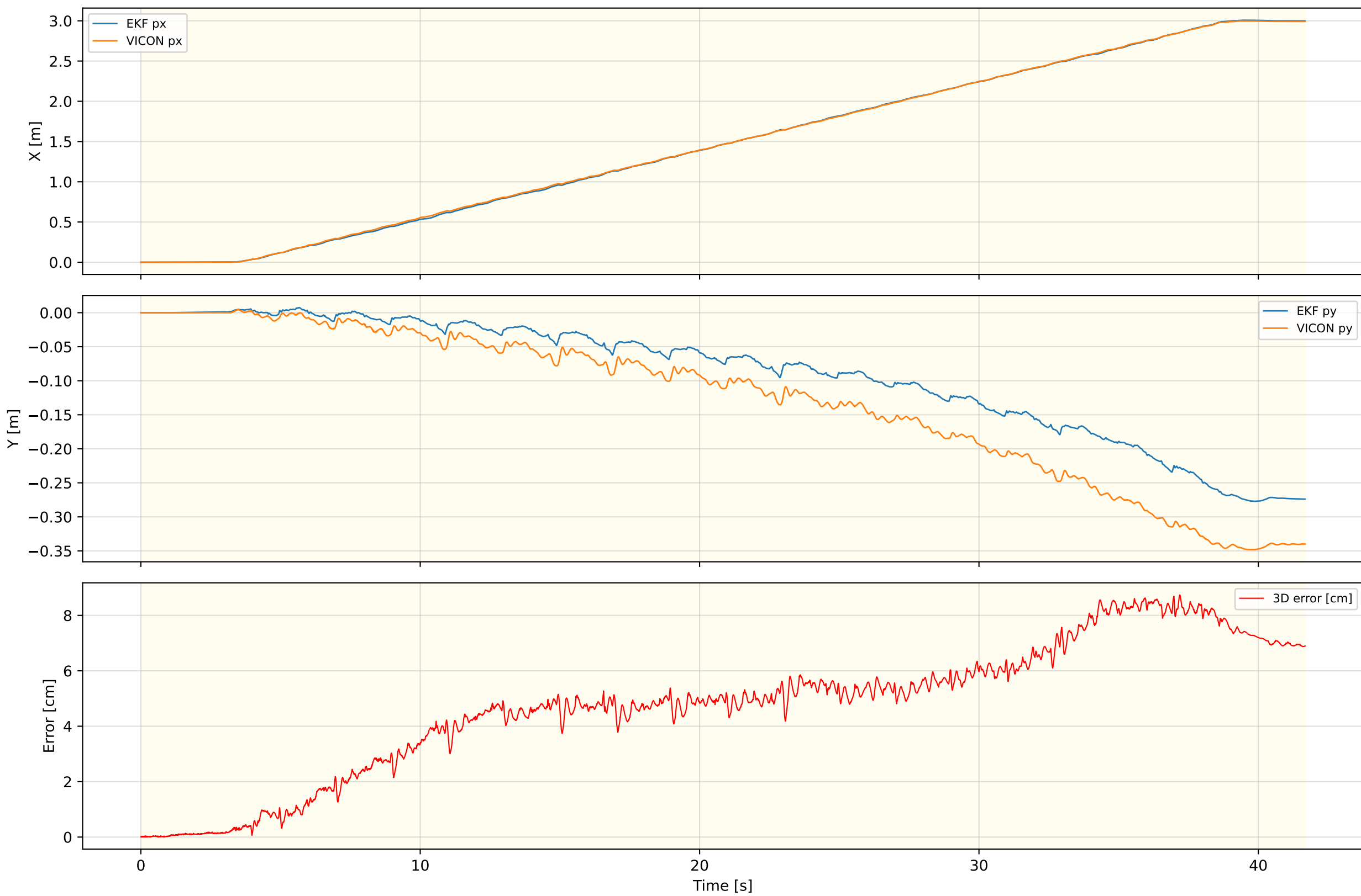
Inner EKF Position — FLAT_MPC_NEW_REAL_5
