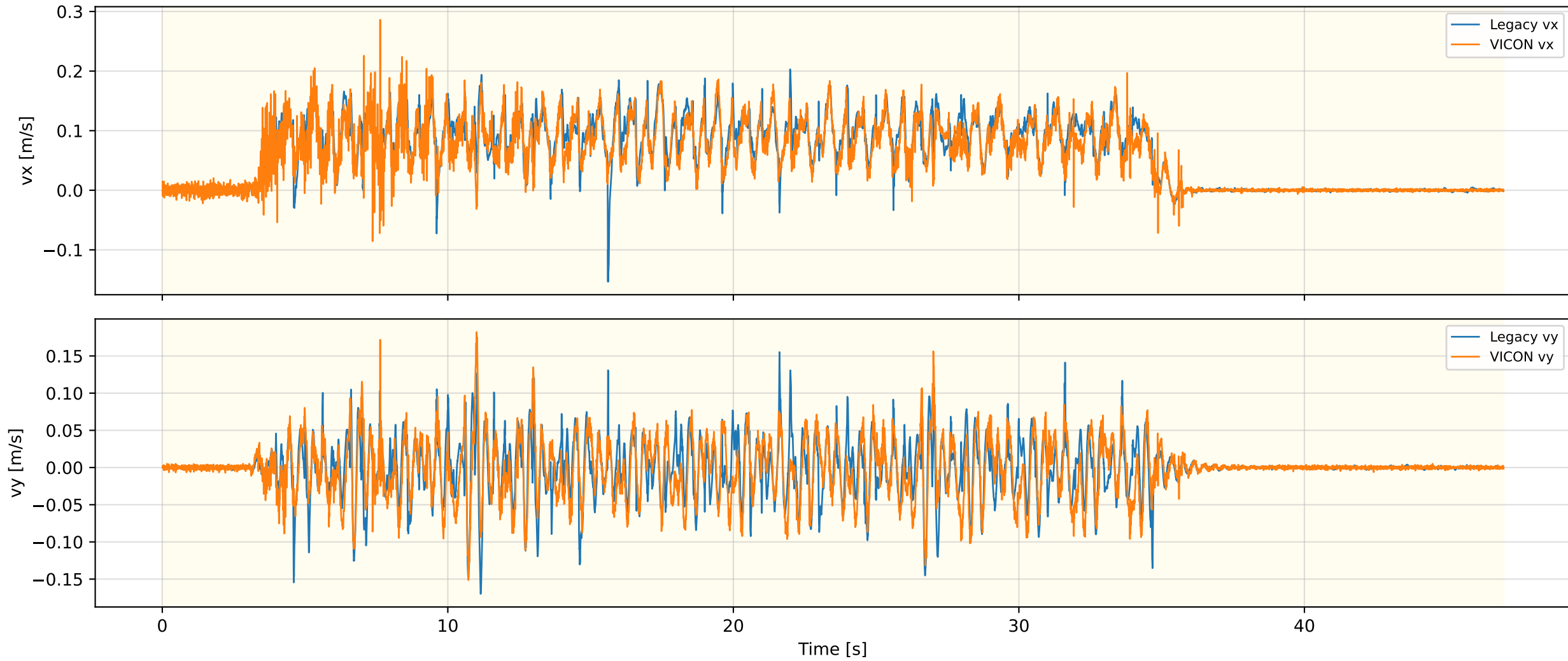
Legacy Odometry Velocity — FLAT_MPC_OLD_REAL_1
