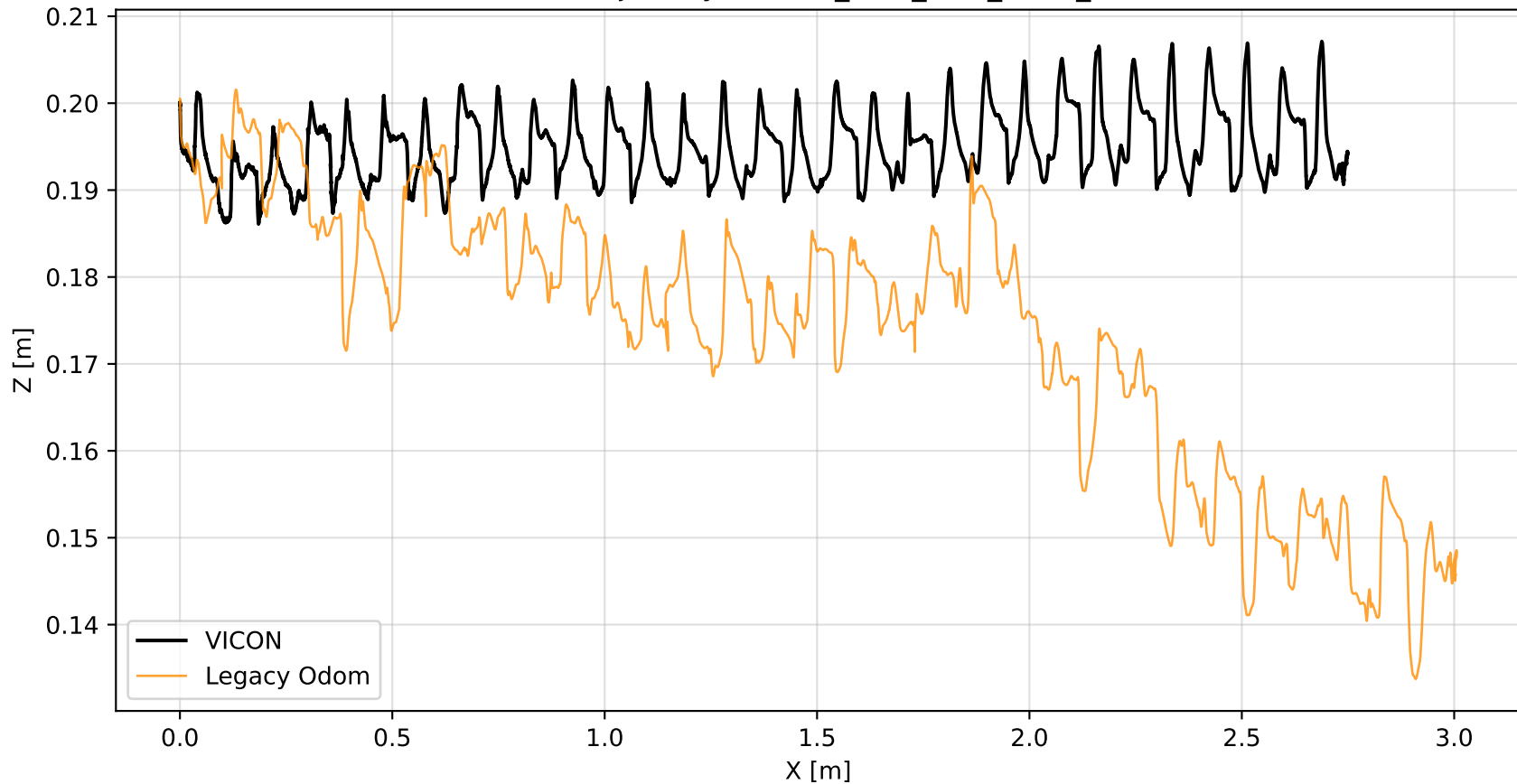
XZ Trajectory — FLAT_MPC_OLD_REAL_1
