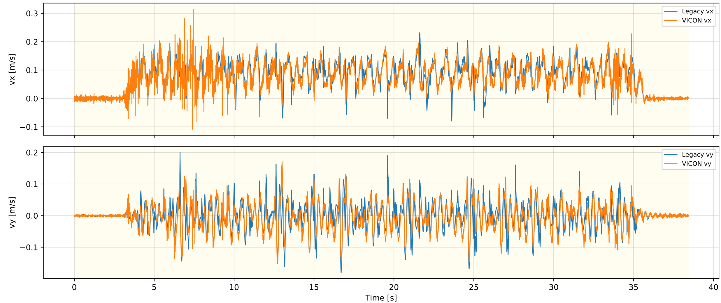
Legacy Odometry Velocity — FLAT_MPC_OLD_REAL_2
