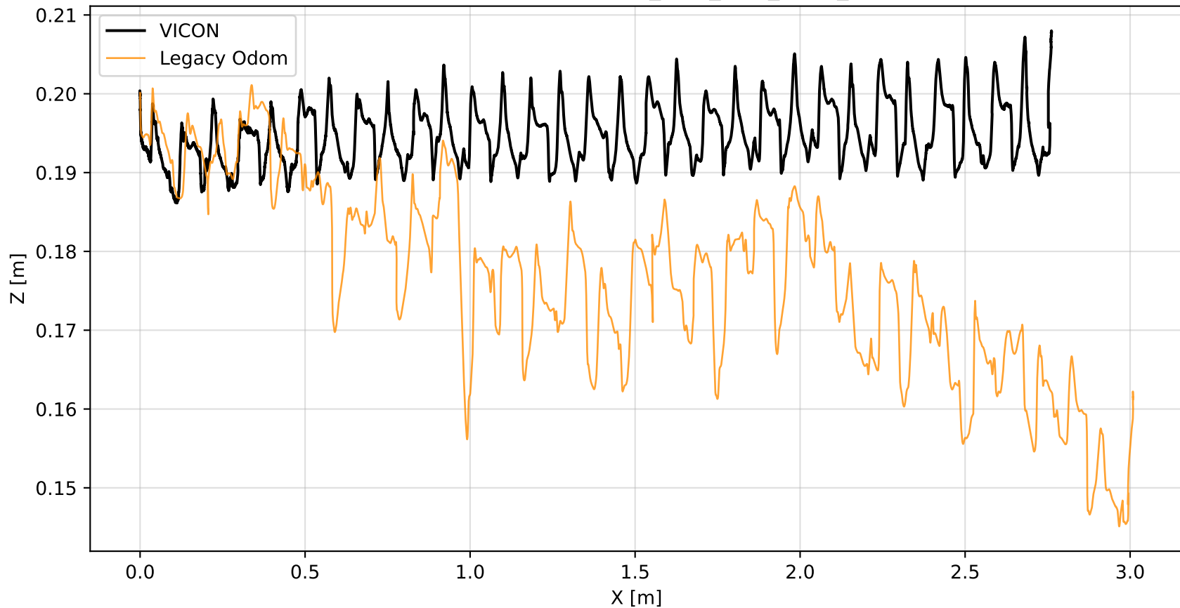
XZ Trajectory — FLAT_MPC_OLD_REAL_3
