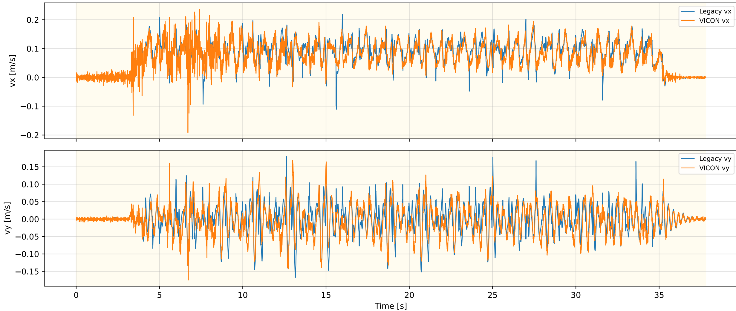
Legacy Odometry Velocity — FLAT_MPC_OLD_REAL_4
