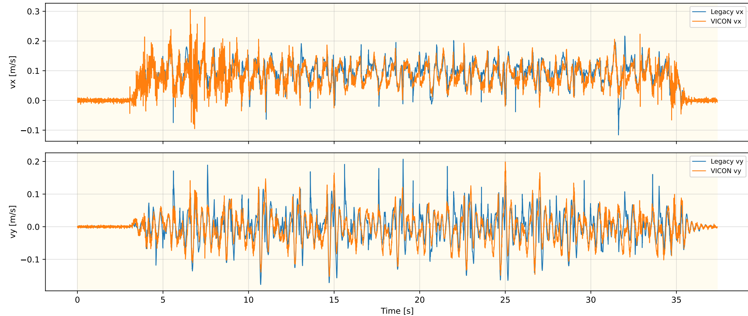
Legacy Odometry Velocity — FLAT_MPC_OLD_REAL_5
