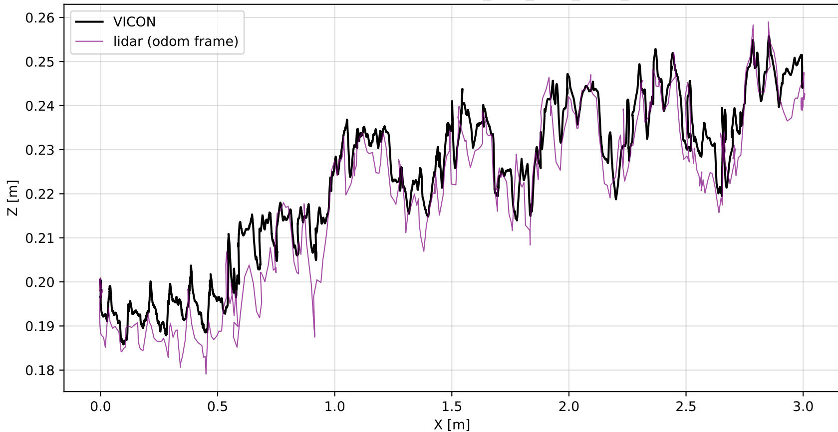
LiDAR XZ Trajectory — OBS_MPC_NEW_REAL_3
