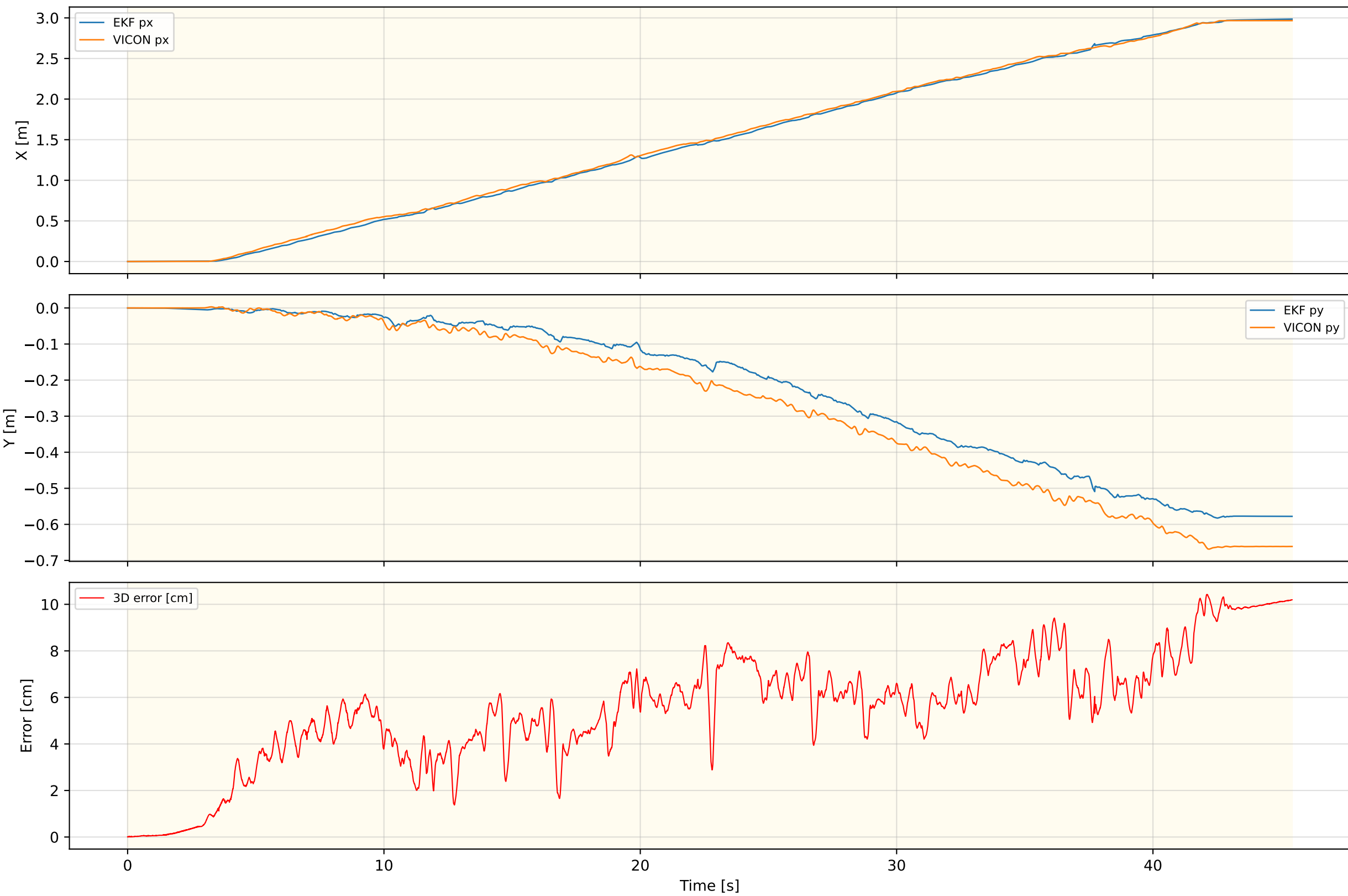
Inner EKF Position — OBS_MPC_NEW_REAL_4
