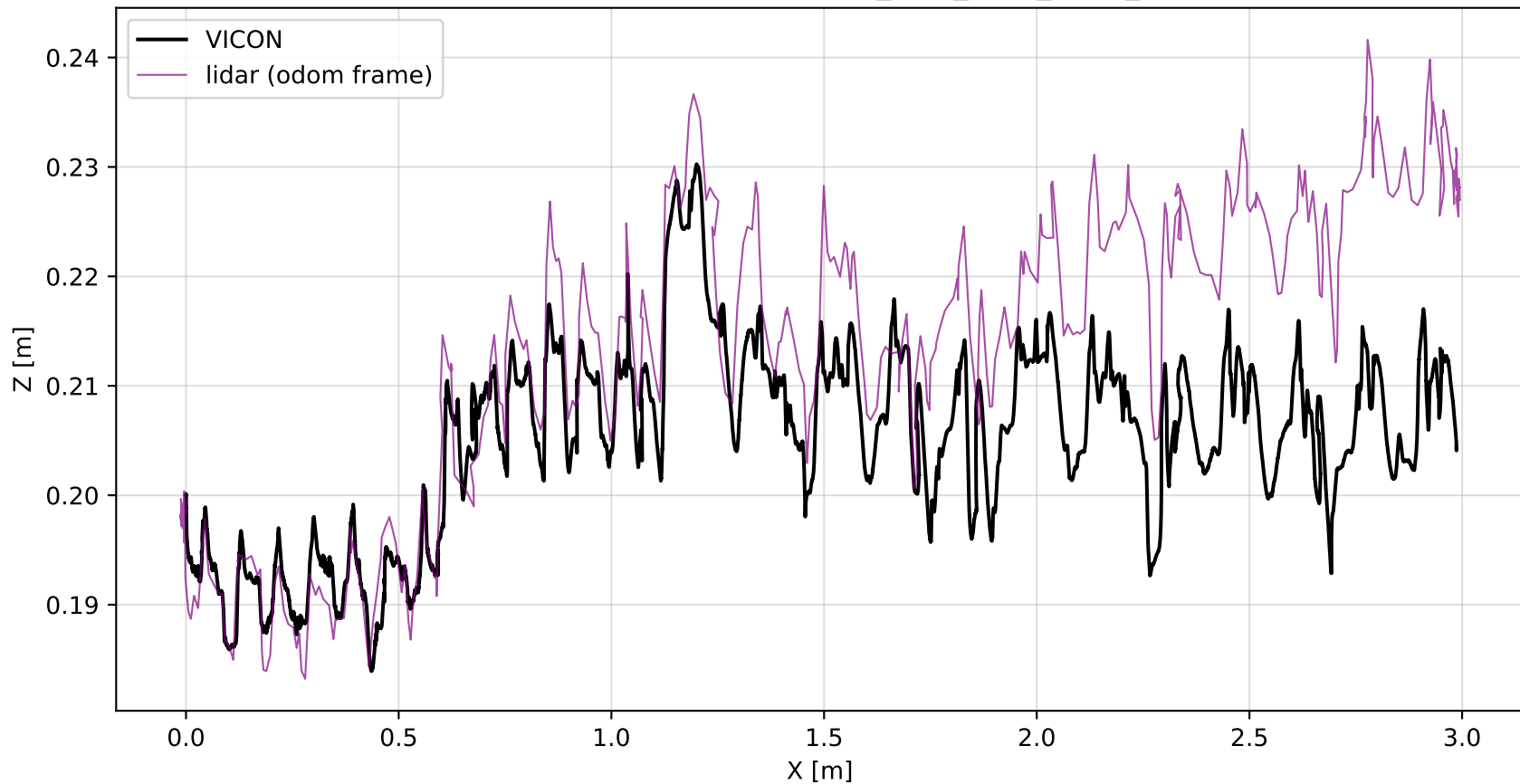
LiDAR XZ Trajectory — OBS_MPC_NEW_REAL_6
