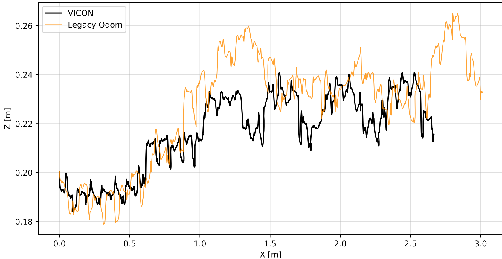
XZ Trajectory — OBS_MPC_OLD_REAL_3
