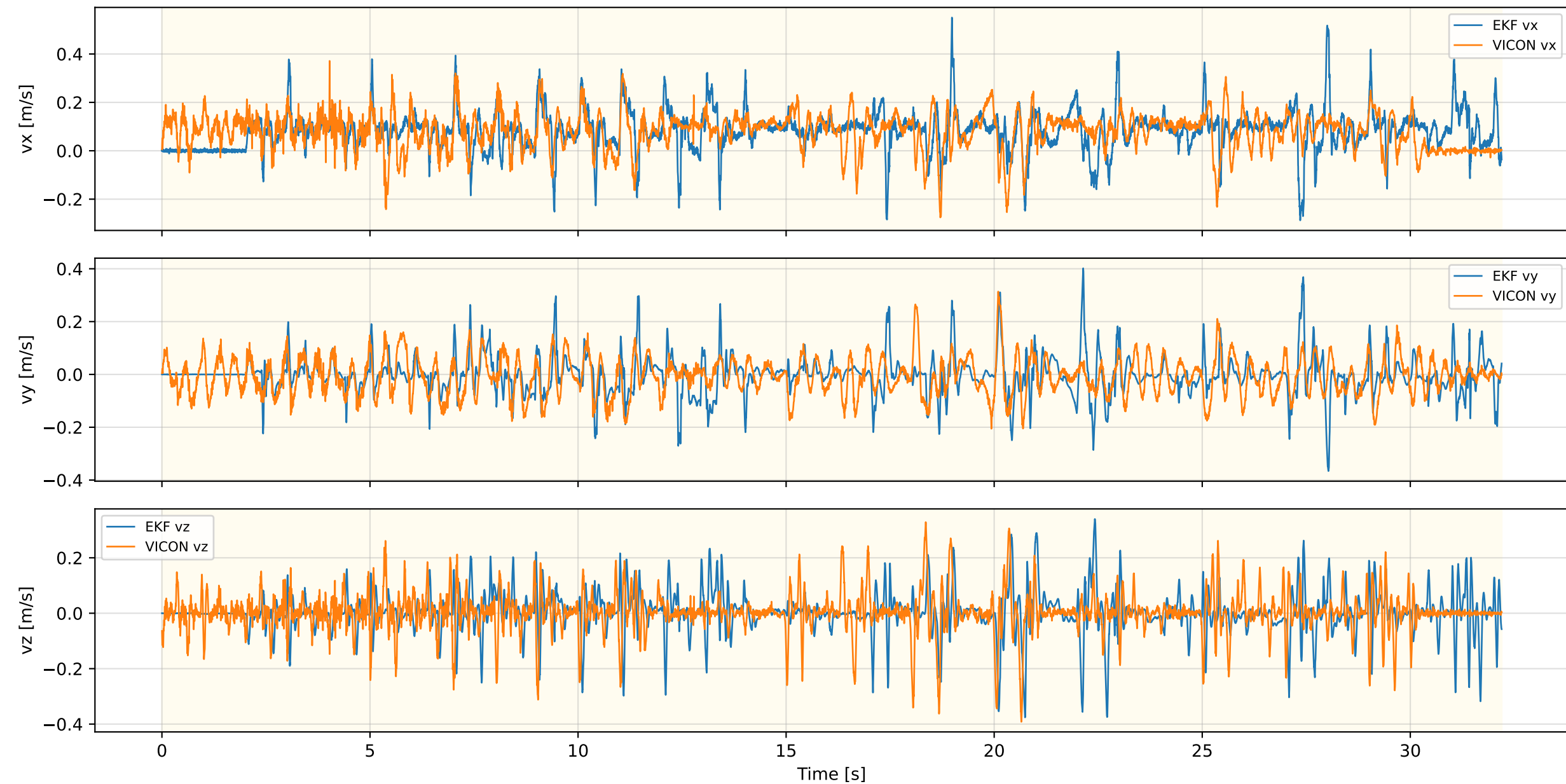
Inner EKF Velocity — RUGG_Walk_NEW_REAL_1
