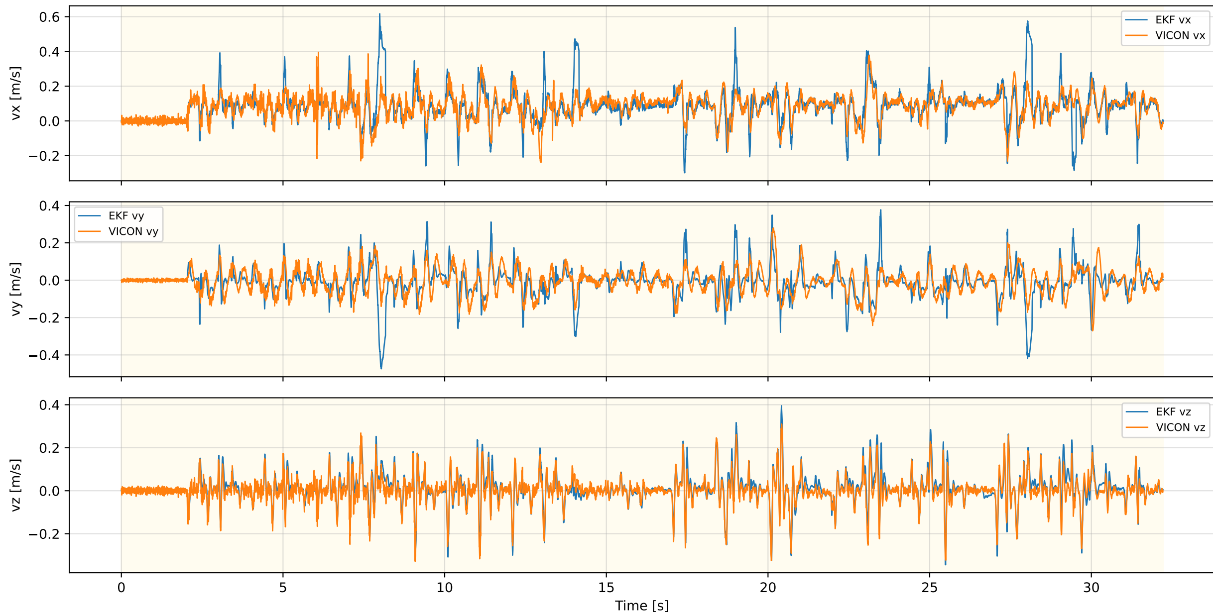
Inner EKF Velocity — RUGG_Walk_NEW_REAL_2
