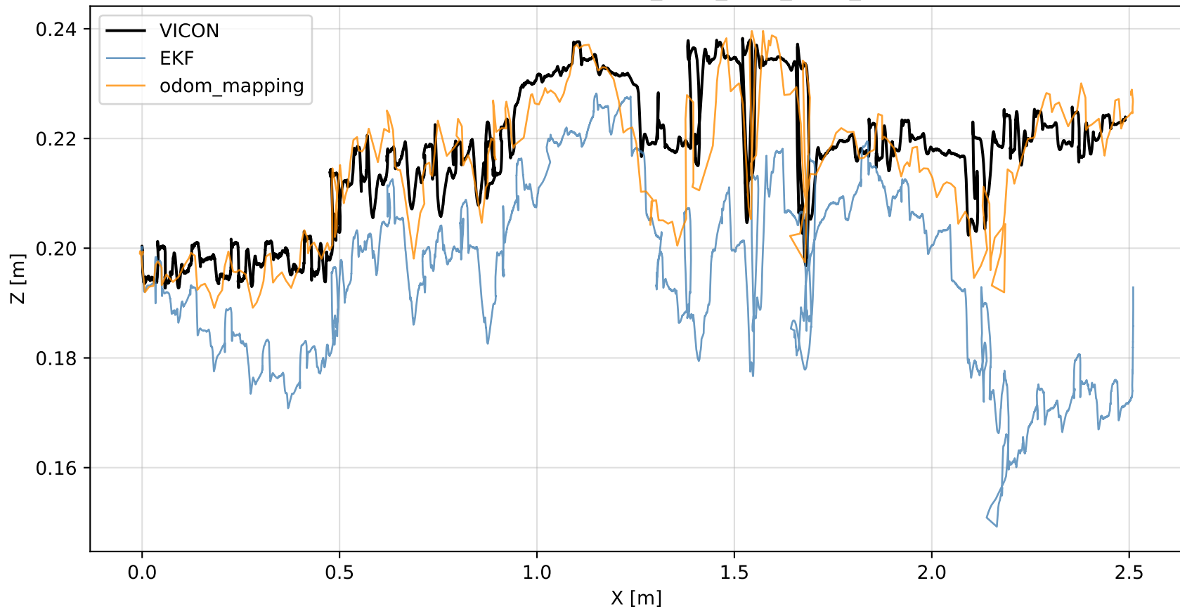
XZ Trajectory — RUGG_Walk_NEW_REAL_5
