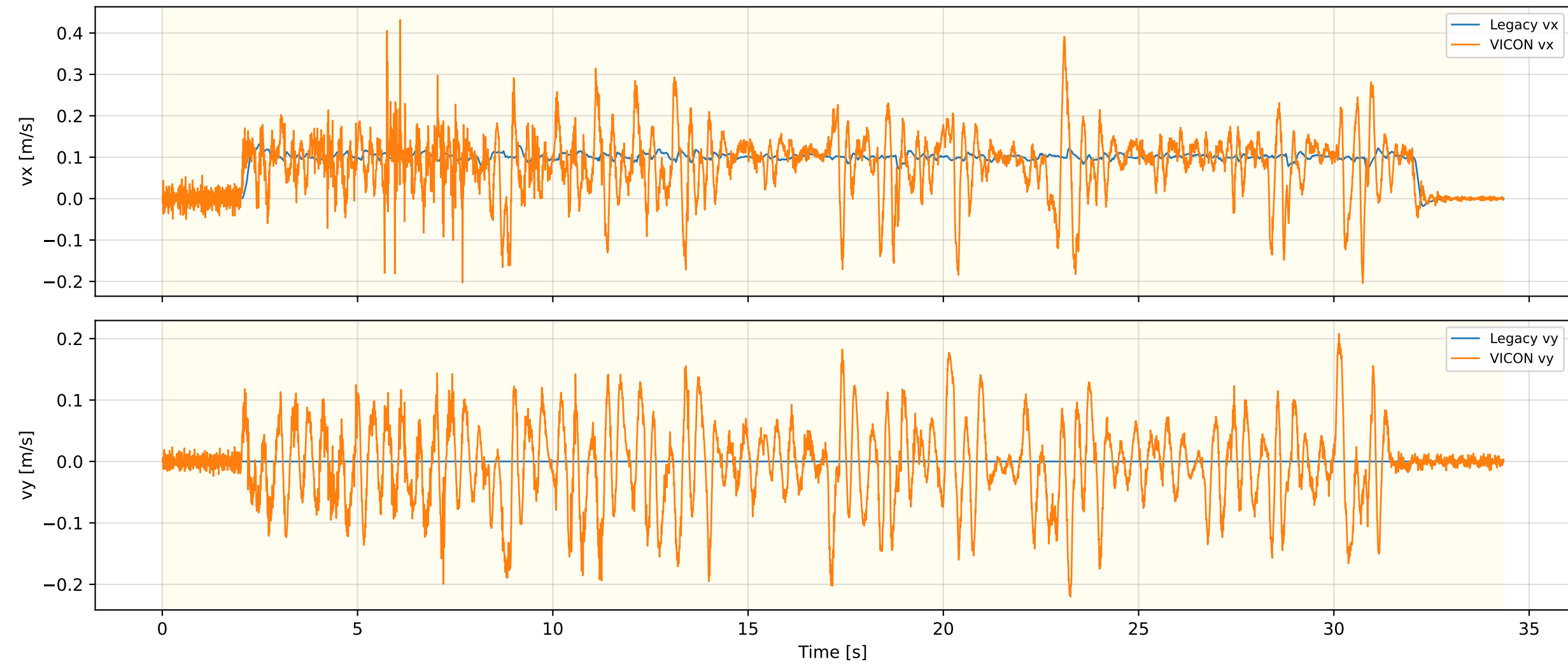
Legacy Odometry Velocity — RUGG_Walk_OLD_REAL_1
