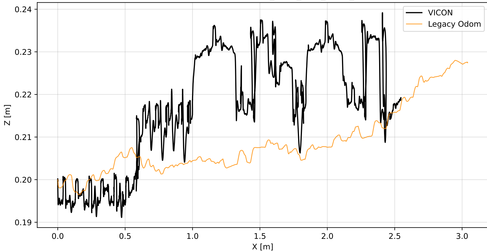
XZ Trajectory — RUGG_Walk_OLD_REAL_1
