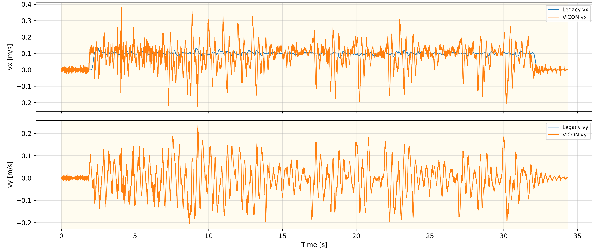
Legacy Odometry Velocity — RUGG_Walk_OLD_REAL_5
