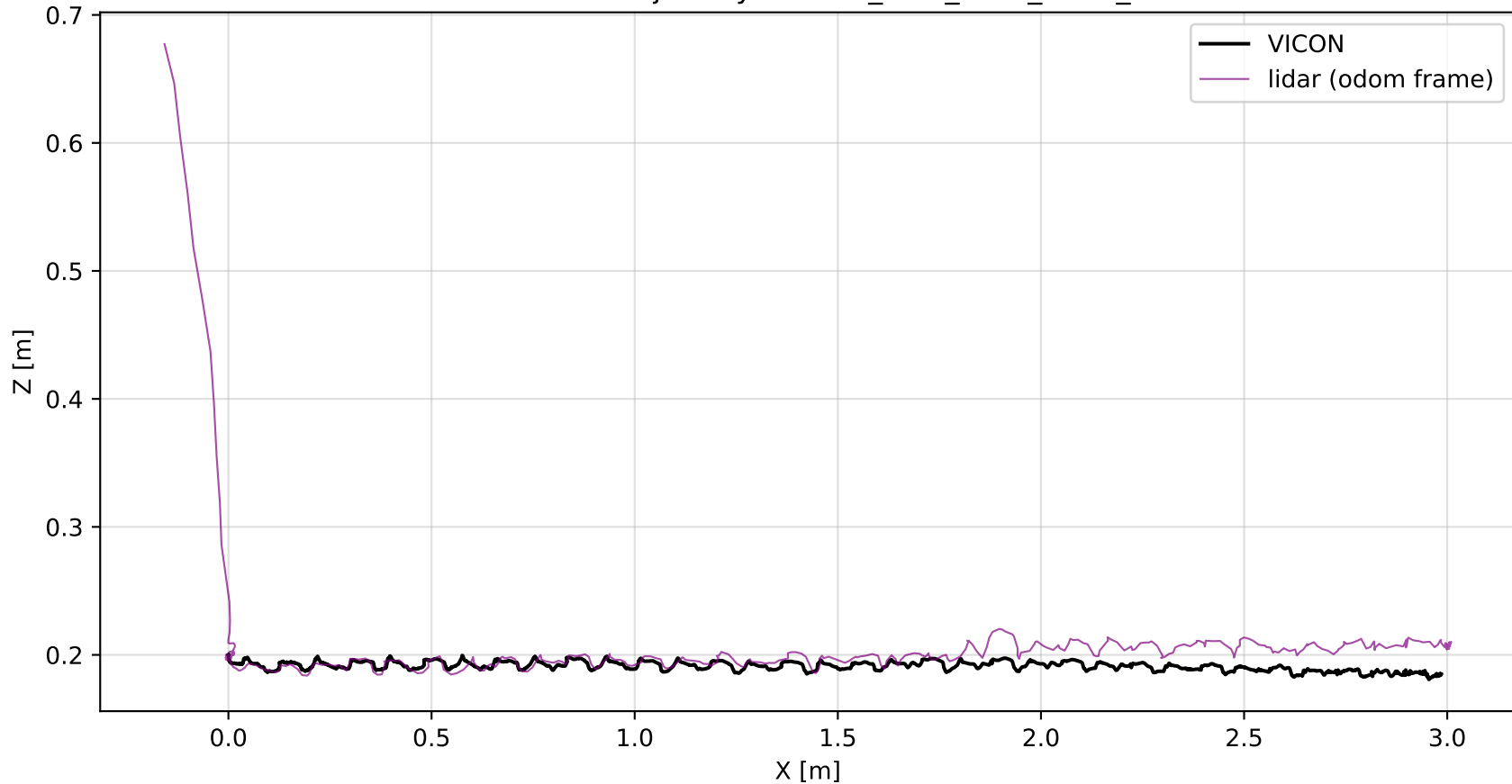
LiDAR XZ Trajectory — FLAT_MPC_NEW_REAL_1
