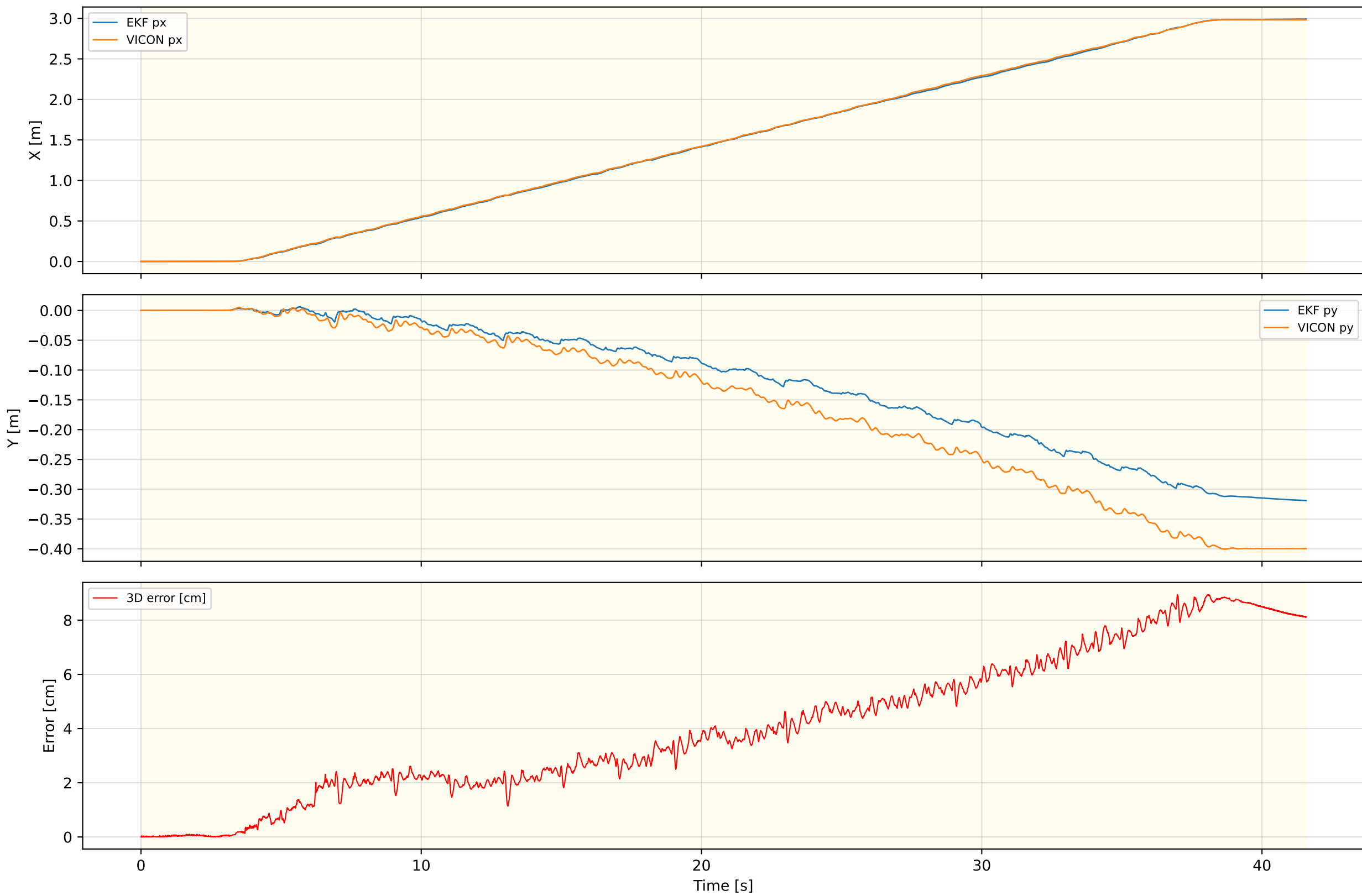
Inner EKF Position — FLAT_MPC_NEW_REAL_2
