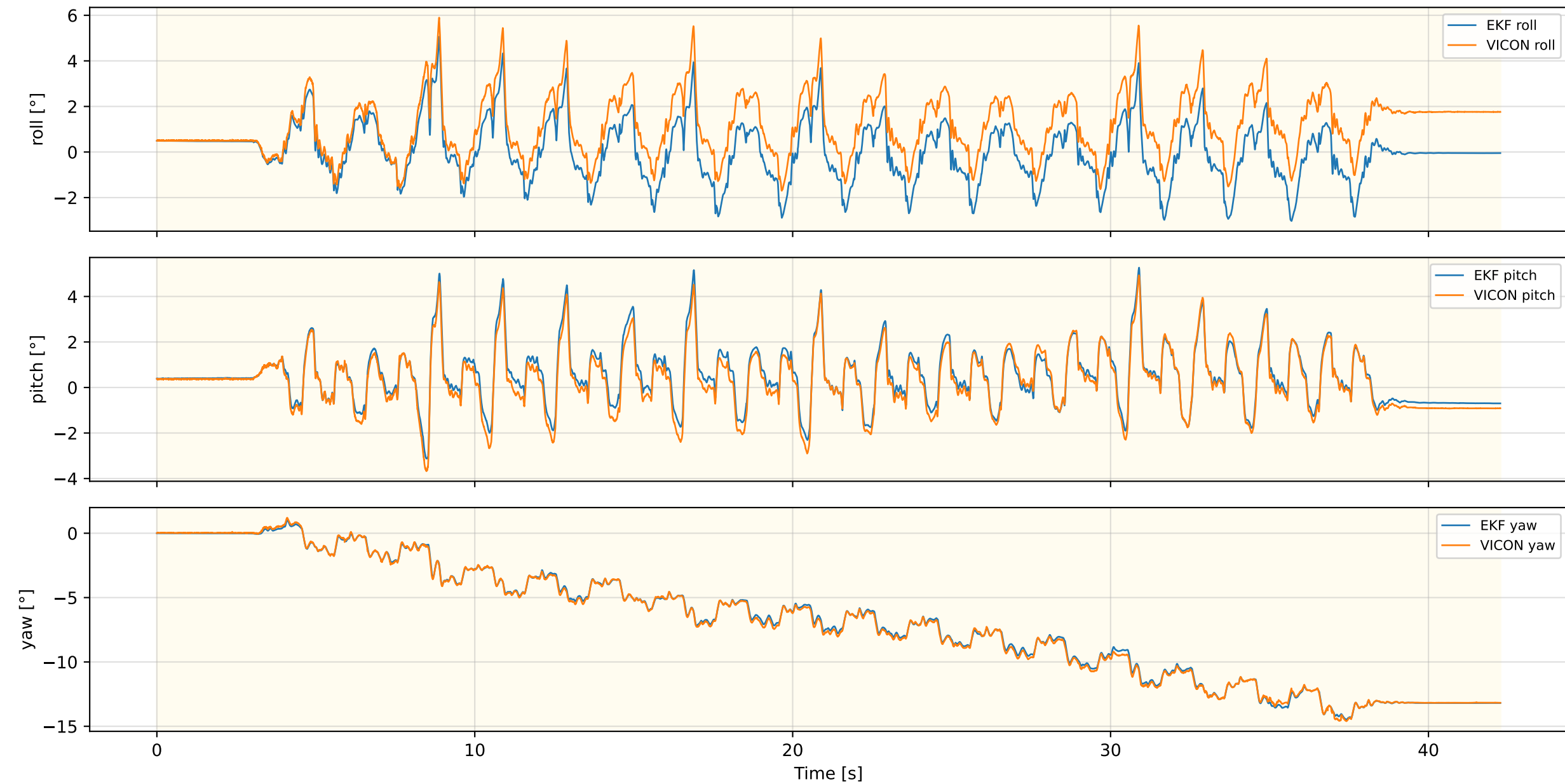
Inner EKF Attitude — FLAT_MPC_NEW_REAL_3
