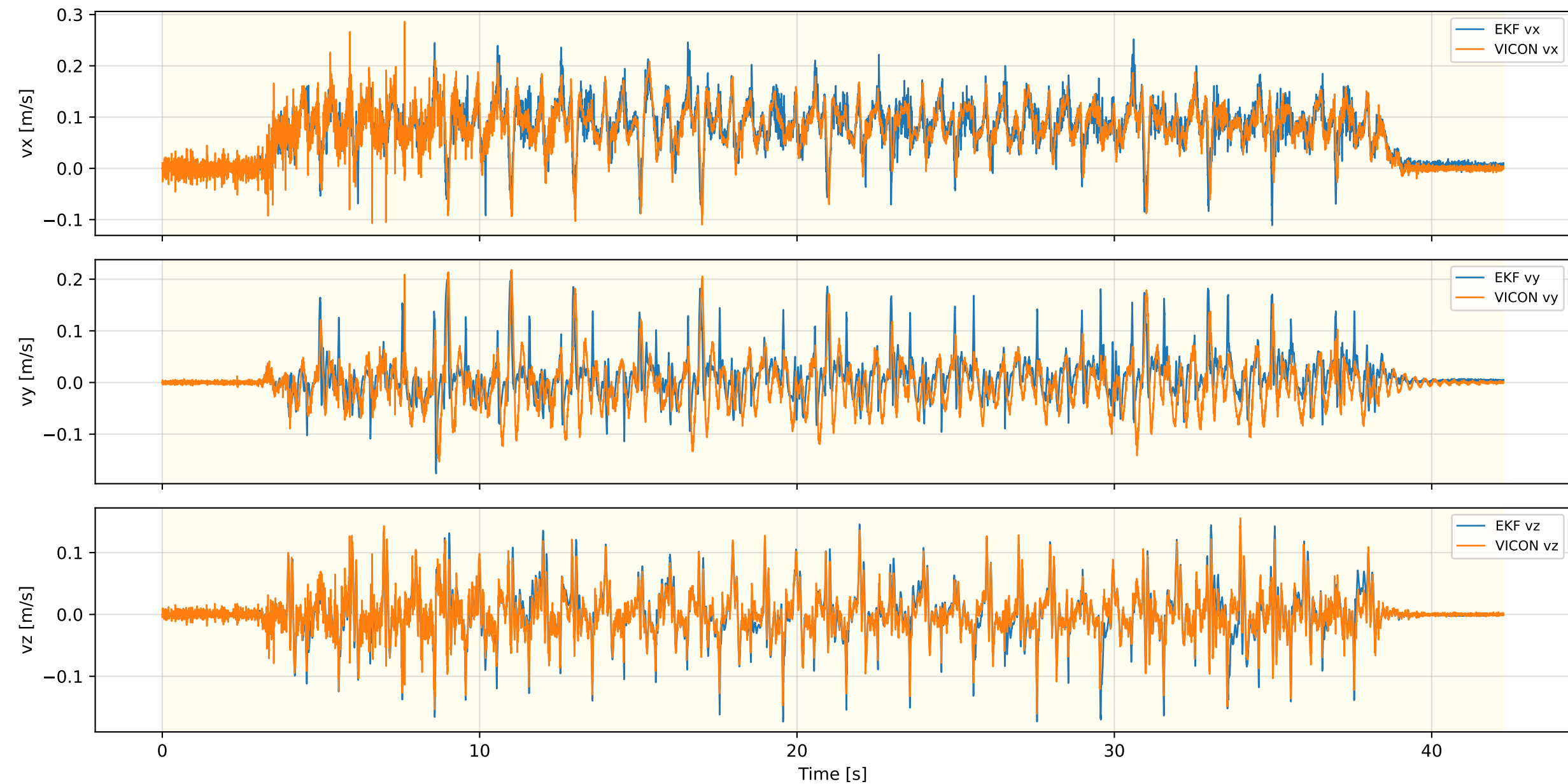
Inner EKF Velocity — FLAT_MPC_NEW_REAL_3
