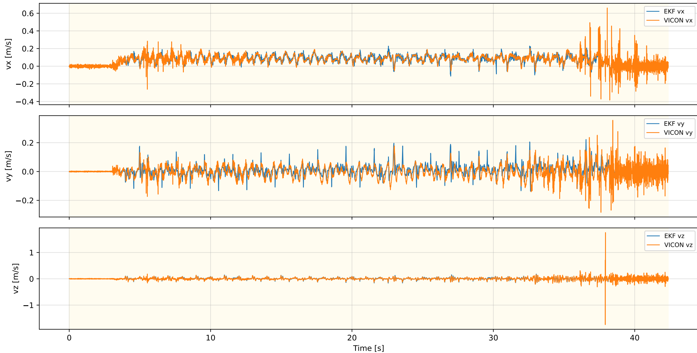
Inner EKF Velocity — FLAT_MPC_NEW_REAL_4
