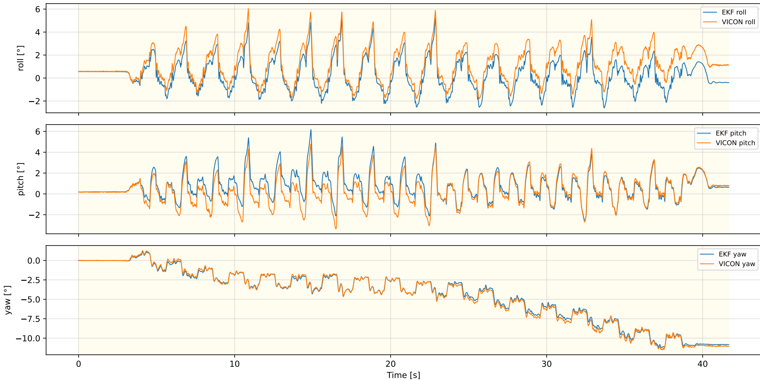
Inner EKF Attitude — FLAT_MPC_NEW_REAL_5
