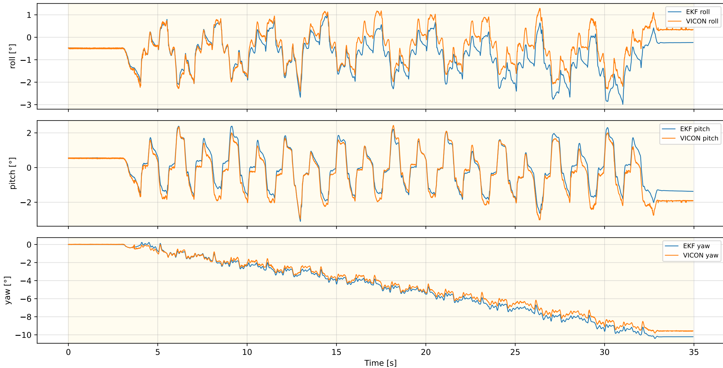
Inner EKF Attitude — FLAT_WLW_NEW_REAL_2
