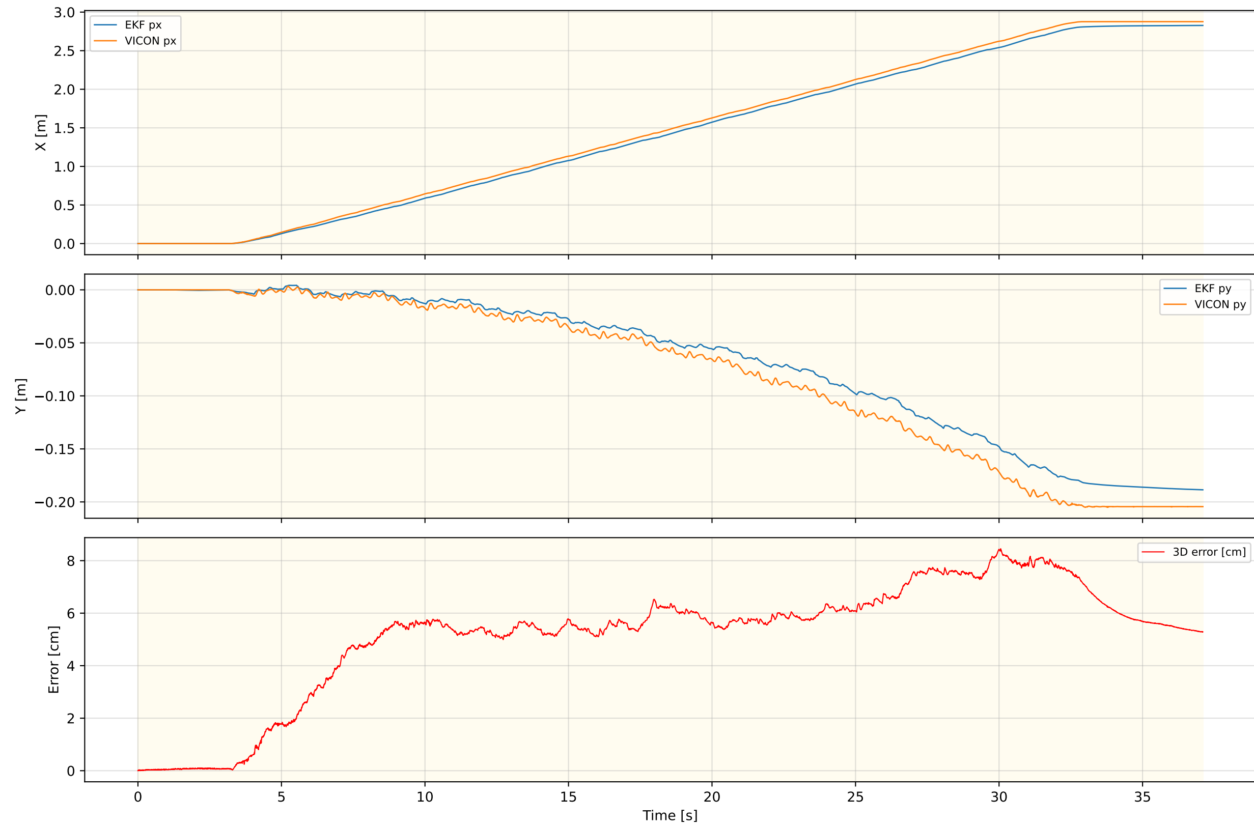
Inner EKF Position — FLAT_WLW_NEW_REAL_3
