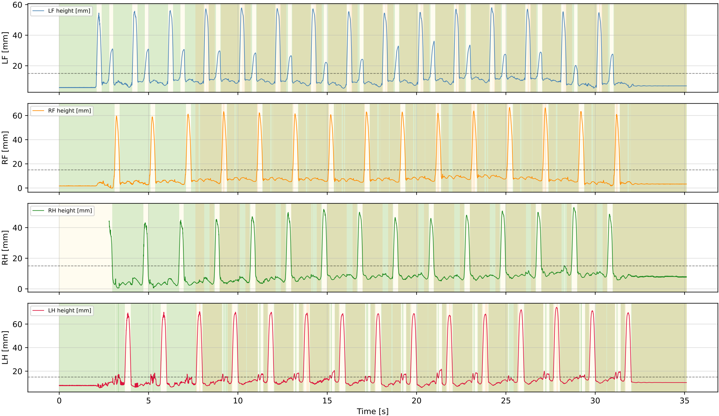
Contact Detection — FLAT_Walk_NEW_REAL_1
