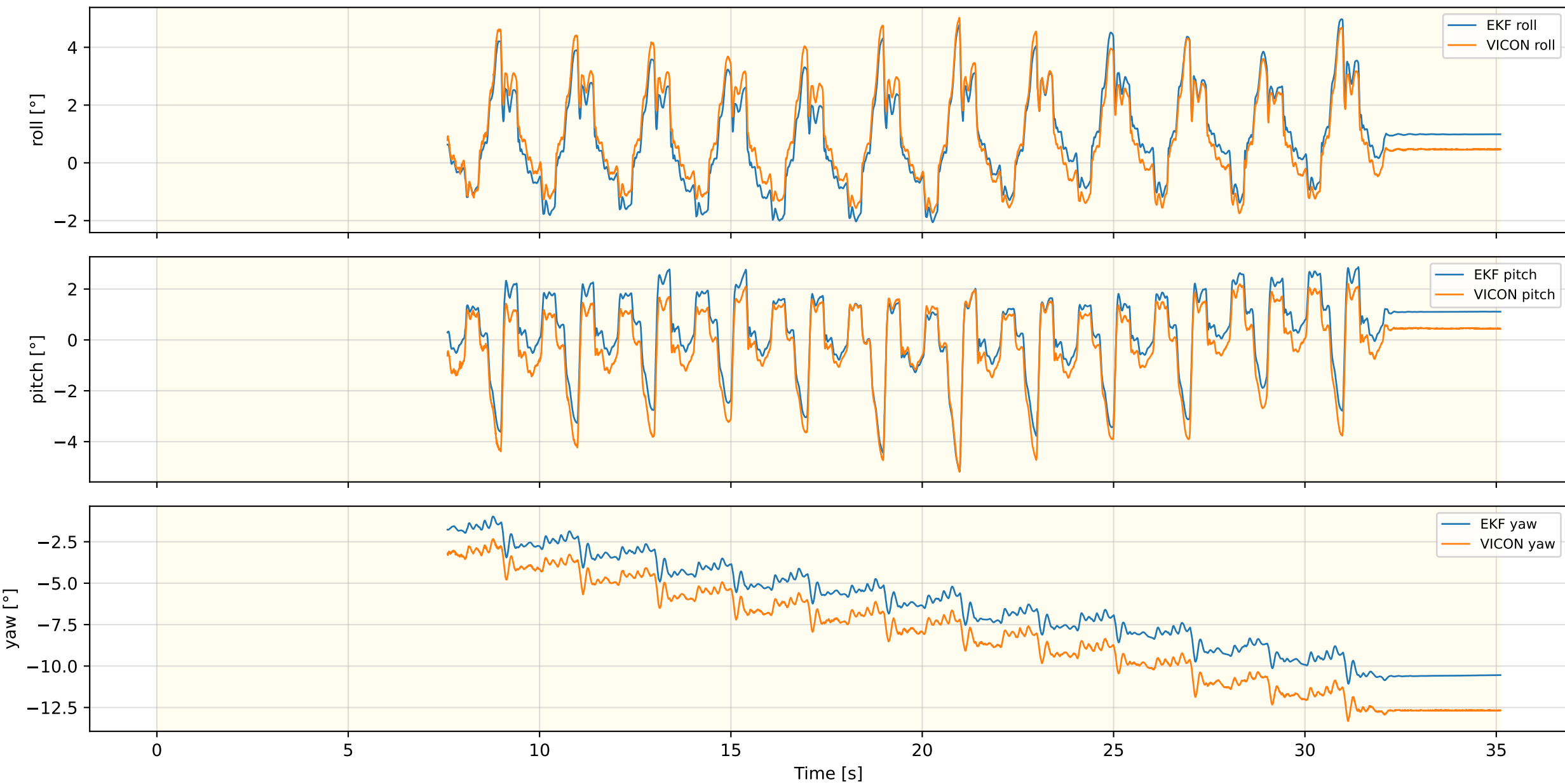
Inner EKF Attitude — FLAT_Walk_NEW_REAL_1
