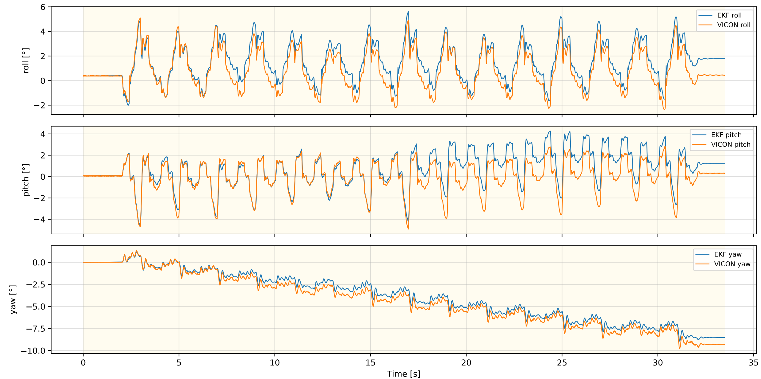
Inner EKF Attitude — FLAT_Walk_NEW_REAL_6
