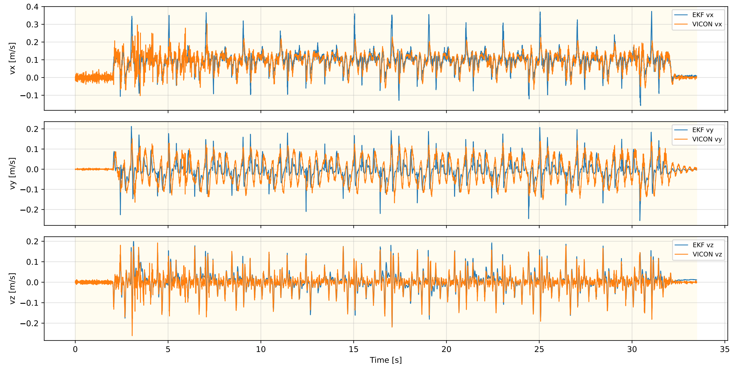
Inner EKF Velocity — FLAT_Walk_NEW_REAL_6
