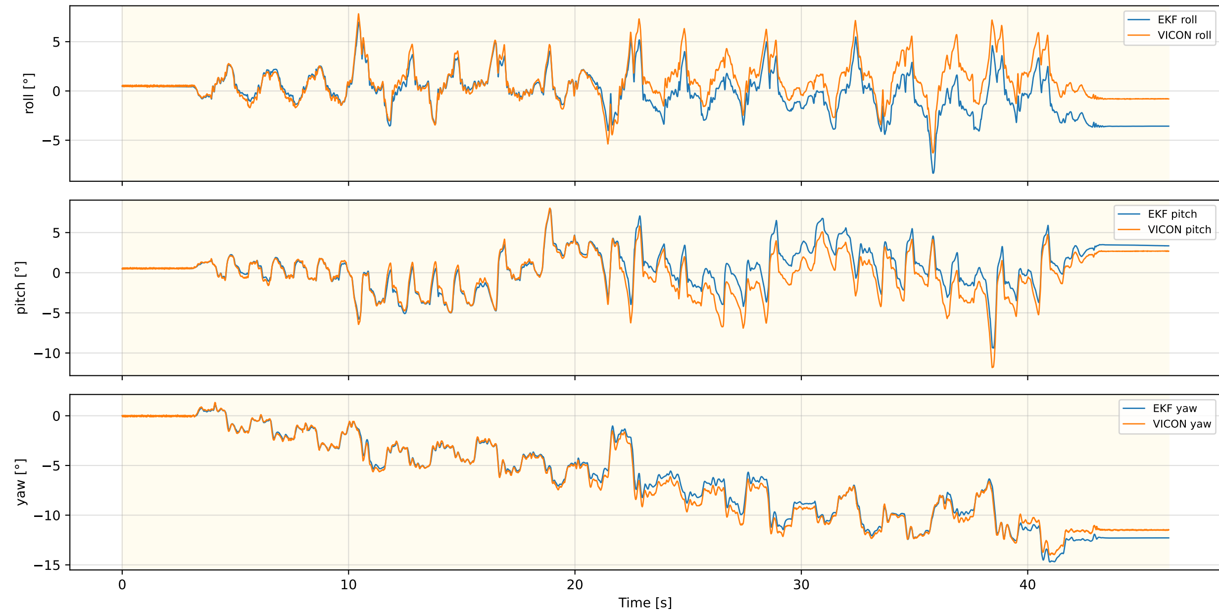
Inner EKF Attitude — OBS_MPC_NEW_REAL_3
