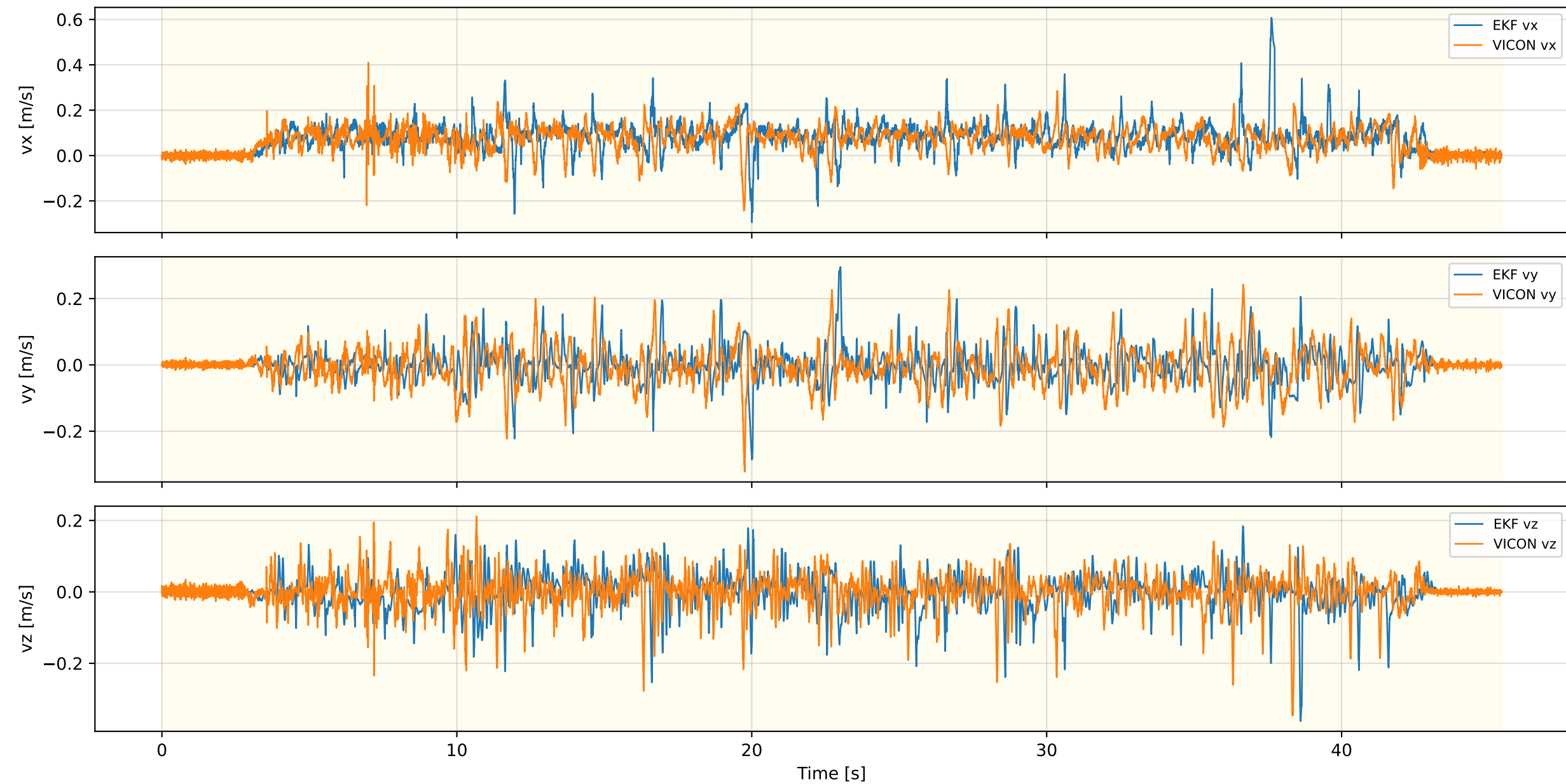
Inner EKF Velocity — OBS_MPC_NEW_REAL_4
