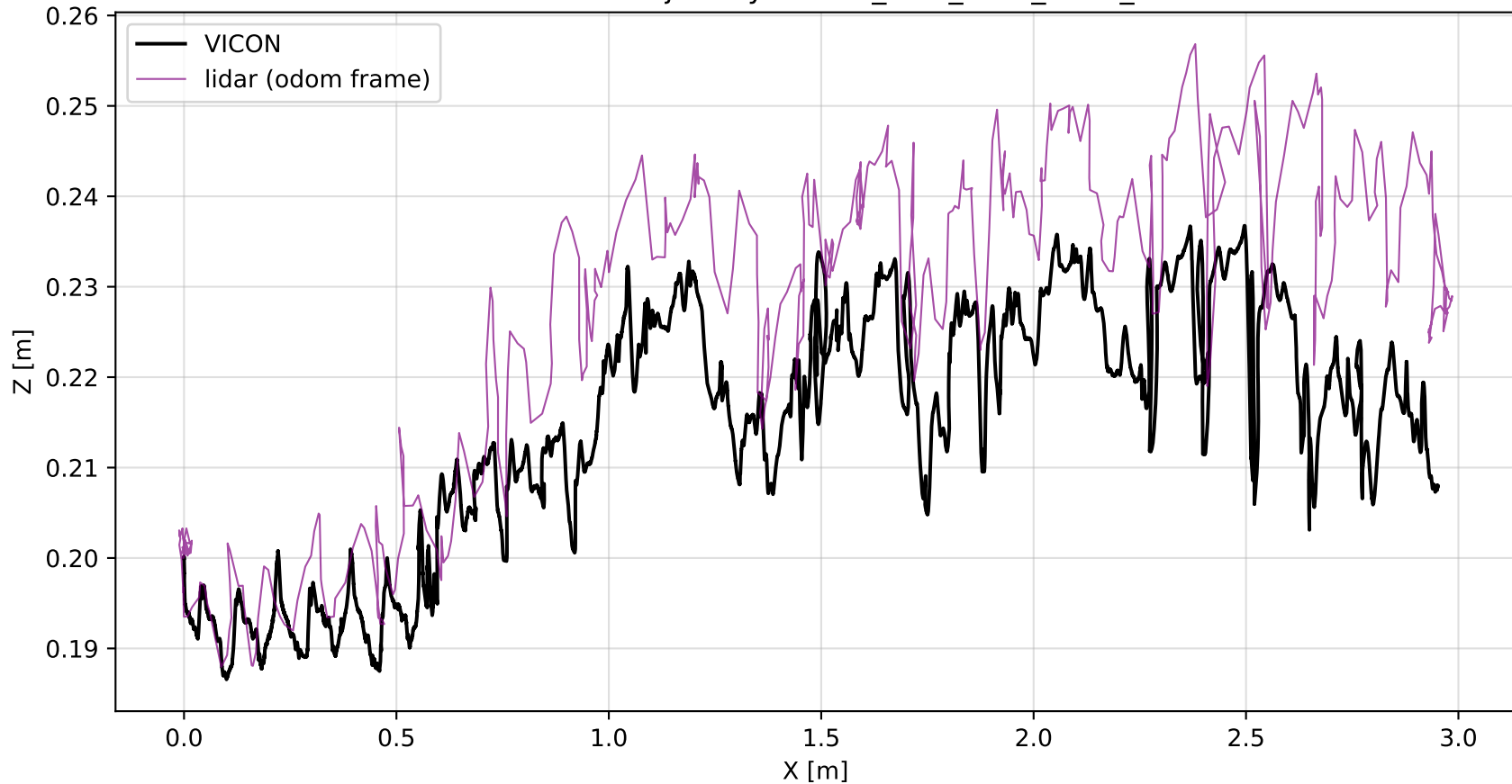
LiDAR XZ Trajectory — OBS_MPC_NEW_REAL_5
