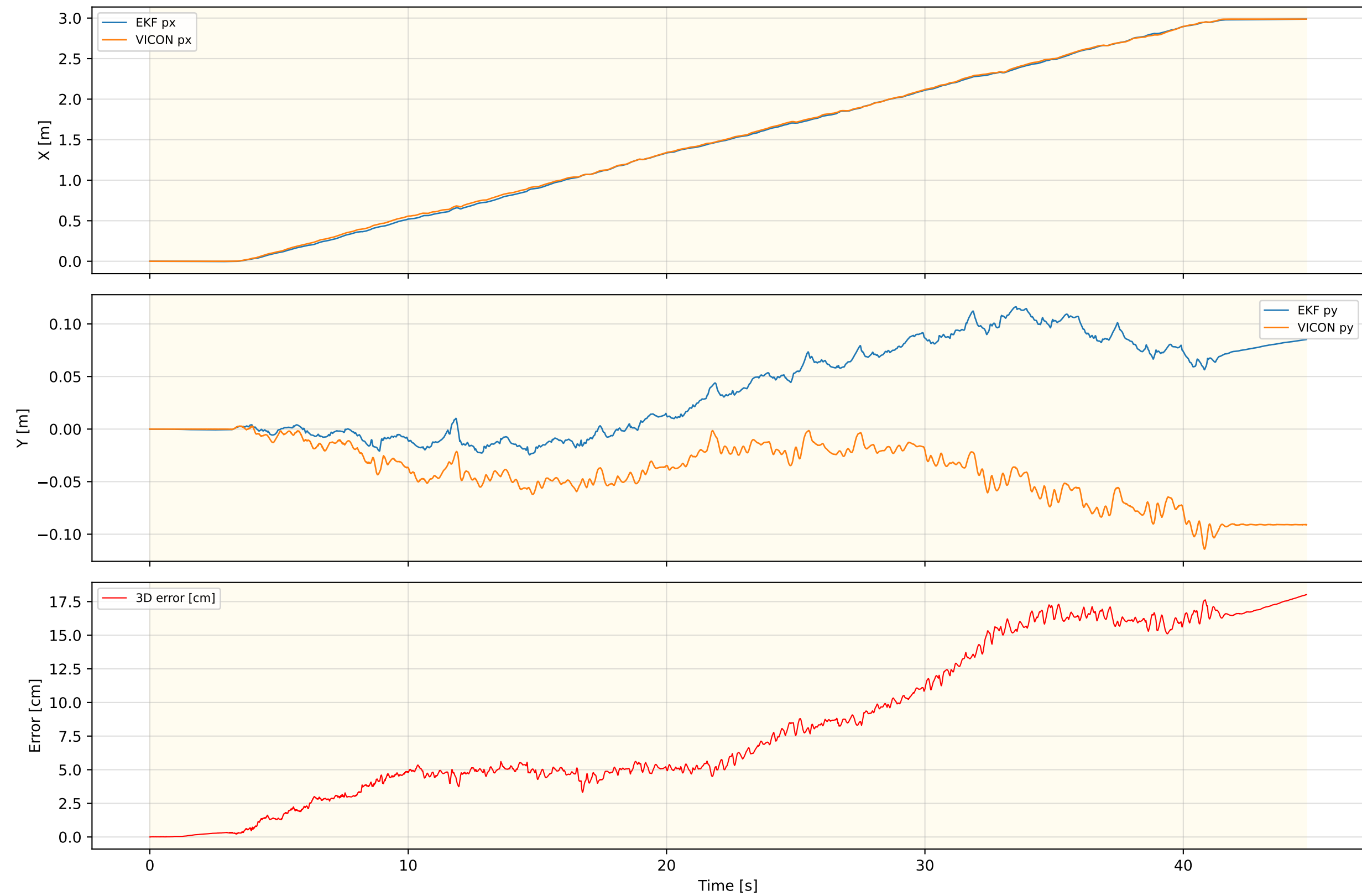
Inner EKF Position — OBS_MPC_NEW_REAL_6
