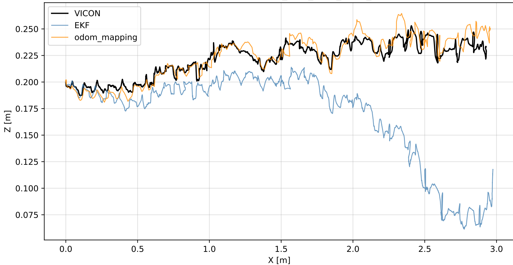
XZ Trajectory — OBS_MPC_NEW_REAL_7
