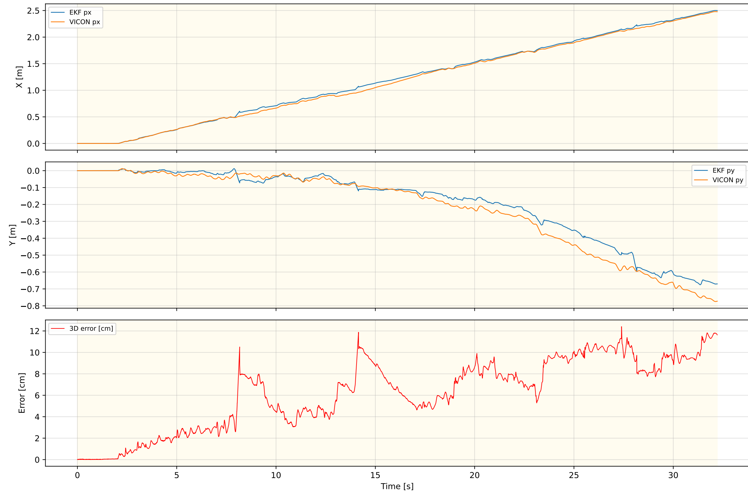
Inner EKF Position — RUGG_Walk_NEW_REAL_2
