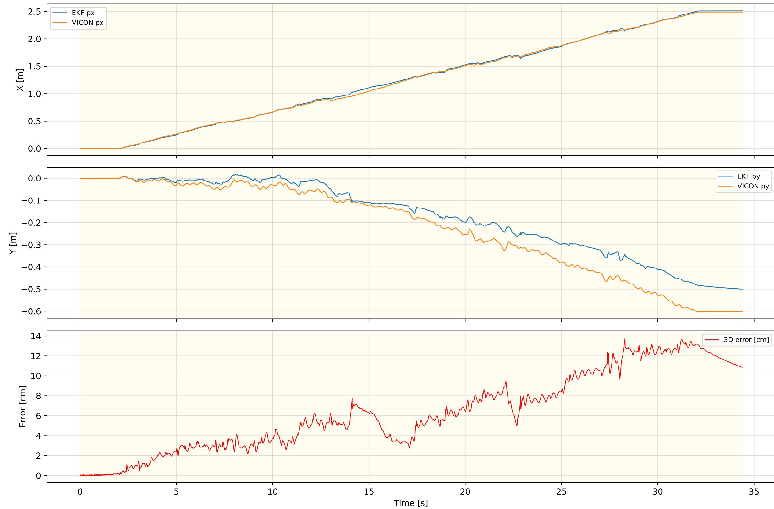
Inner EKF Position — RUGG_Walk_NEW_REAL_5
