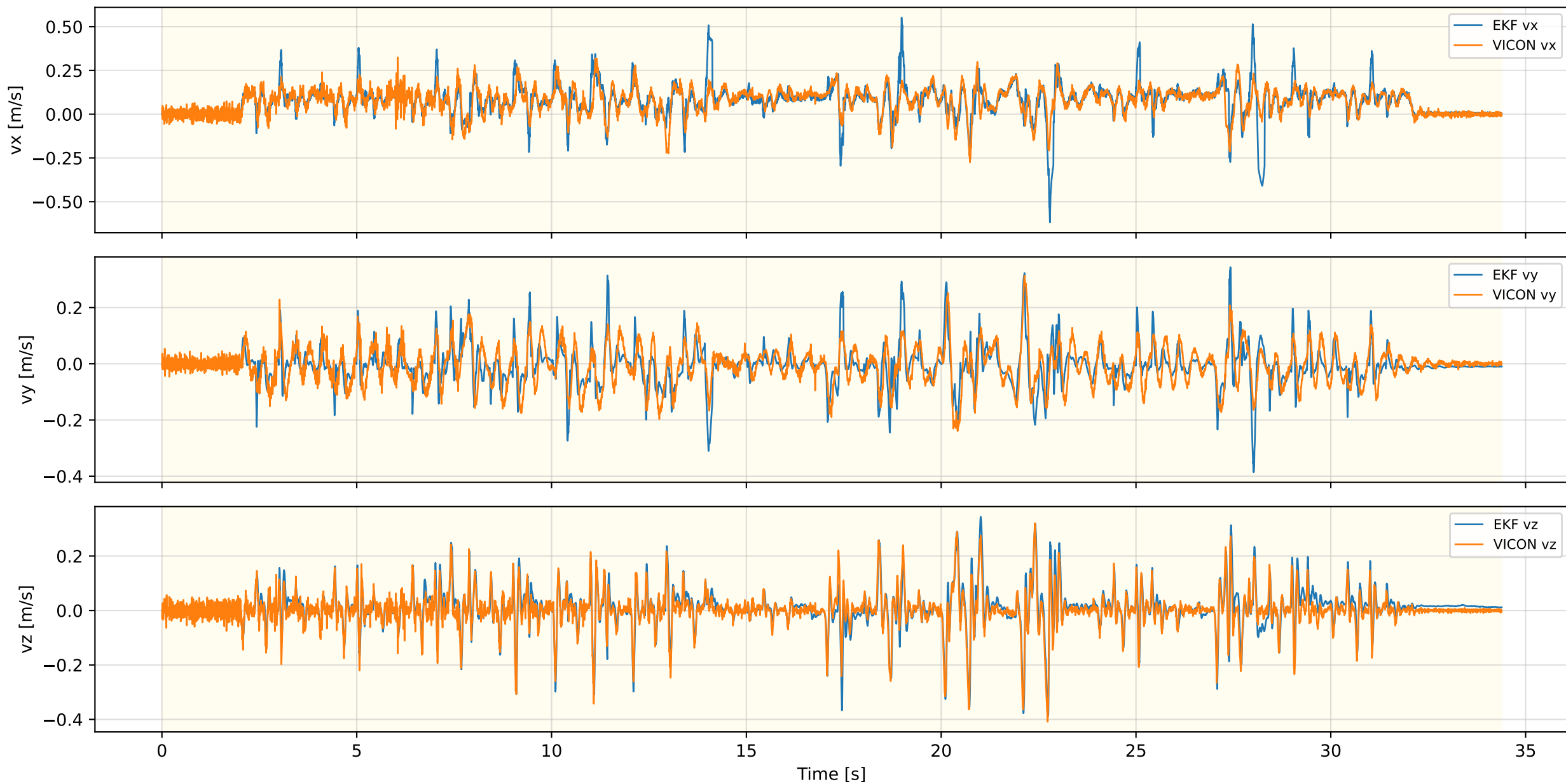
Inner EKF Velocity — RUGG_Walk_NEW_REAL_5
