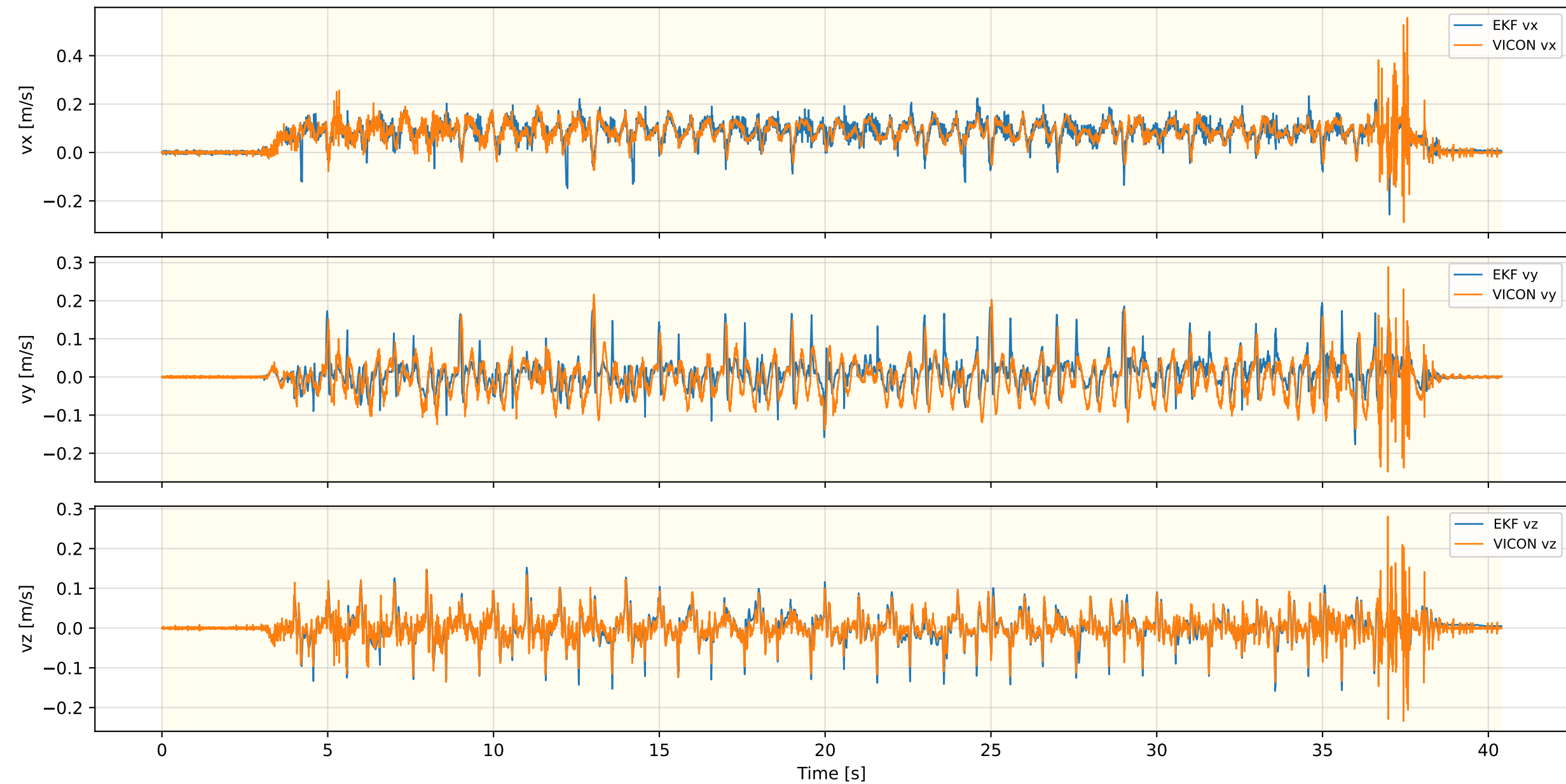
Inner EKF Velocity — FLAT_MPC_NEW_REAL_1
