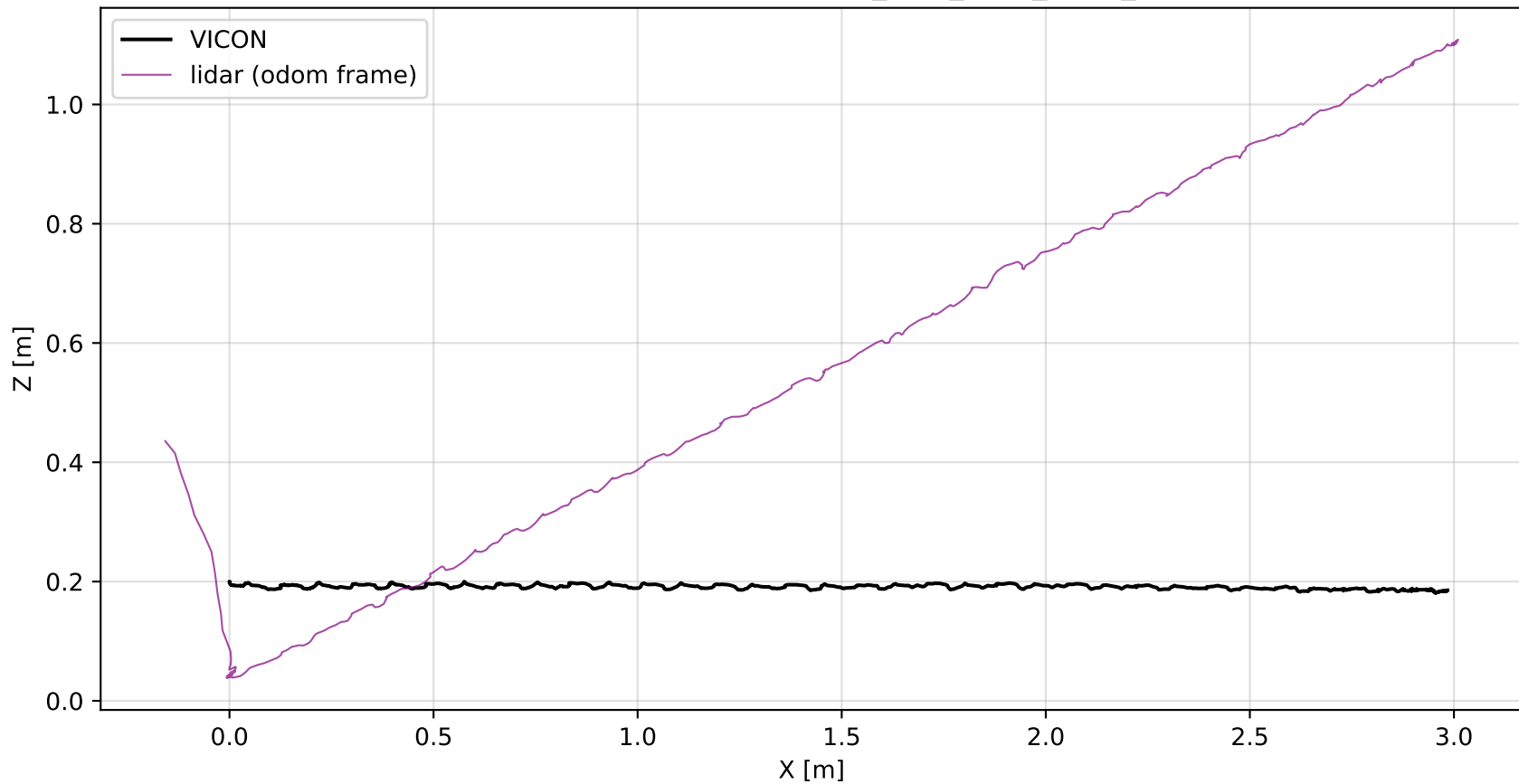
LiDAR XZ Trajectory — FLAT_MPC_NEW_REAL_1
