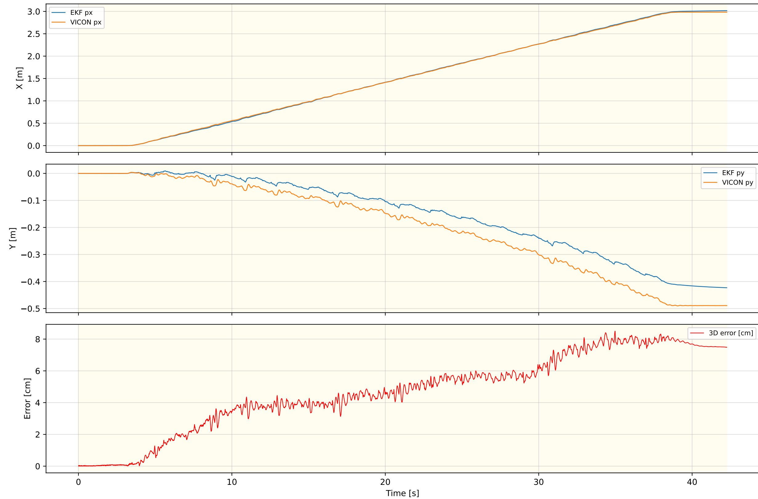
Inner EKF Position — FLAT_MPC_NEW_REAL_3
