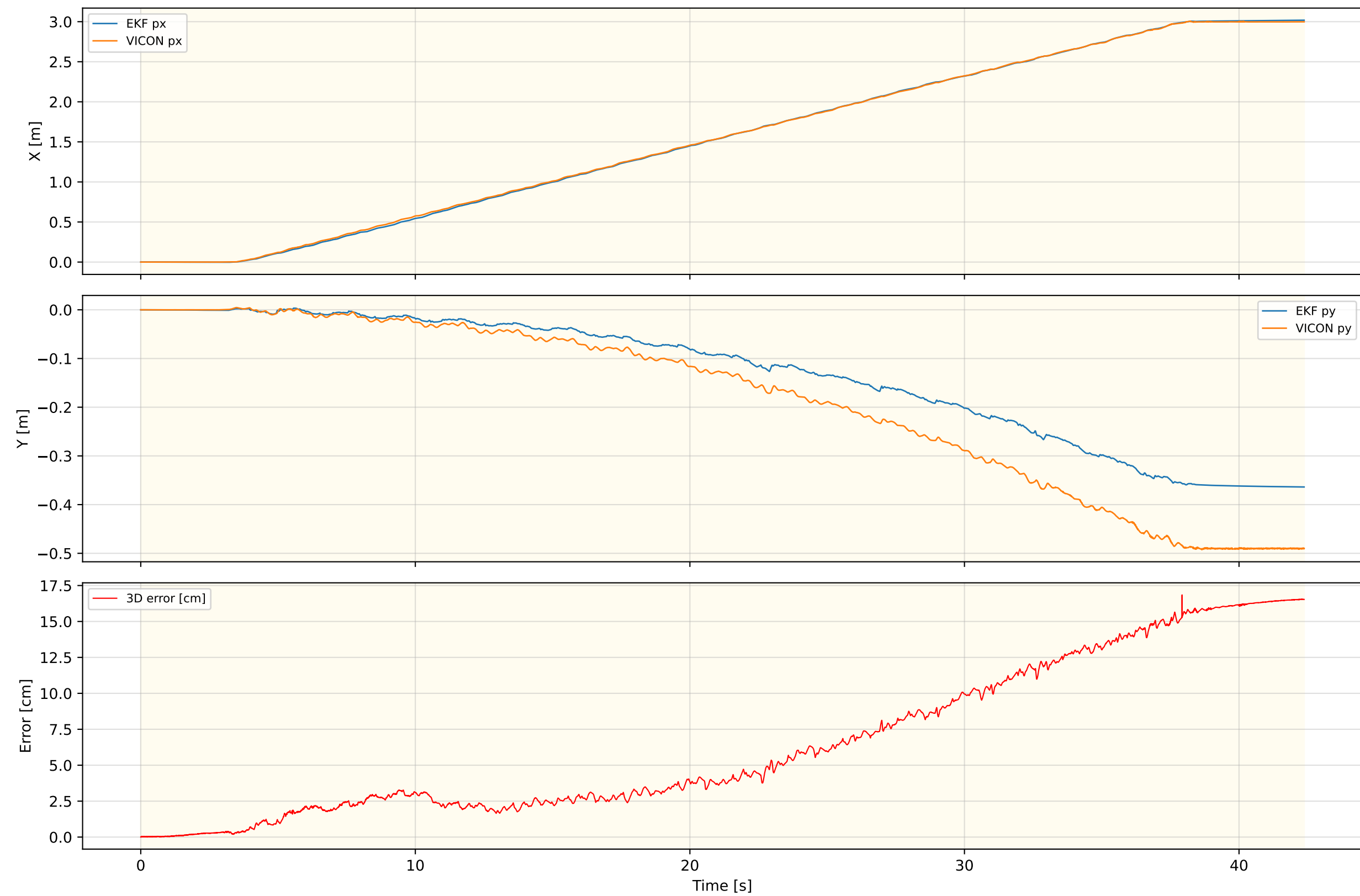
Inner EKF Position — FLAT_MPC_NEW_REAL_4
