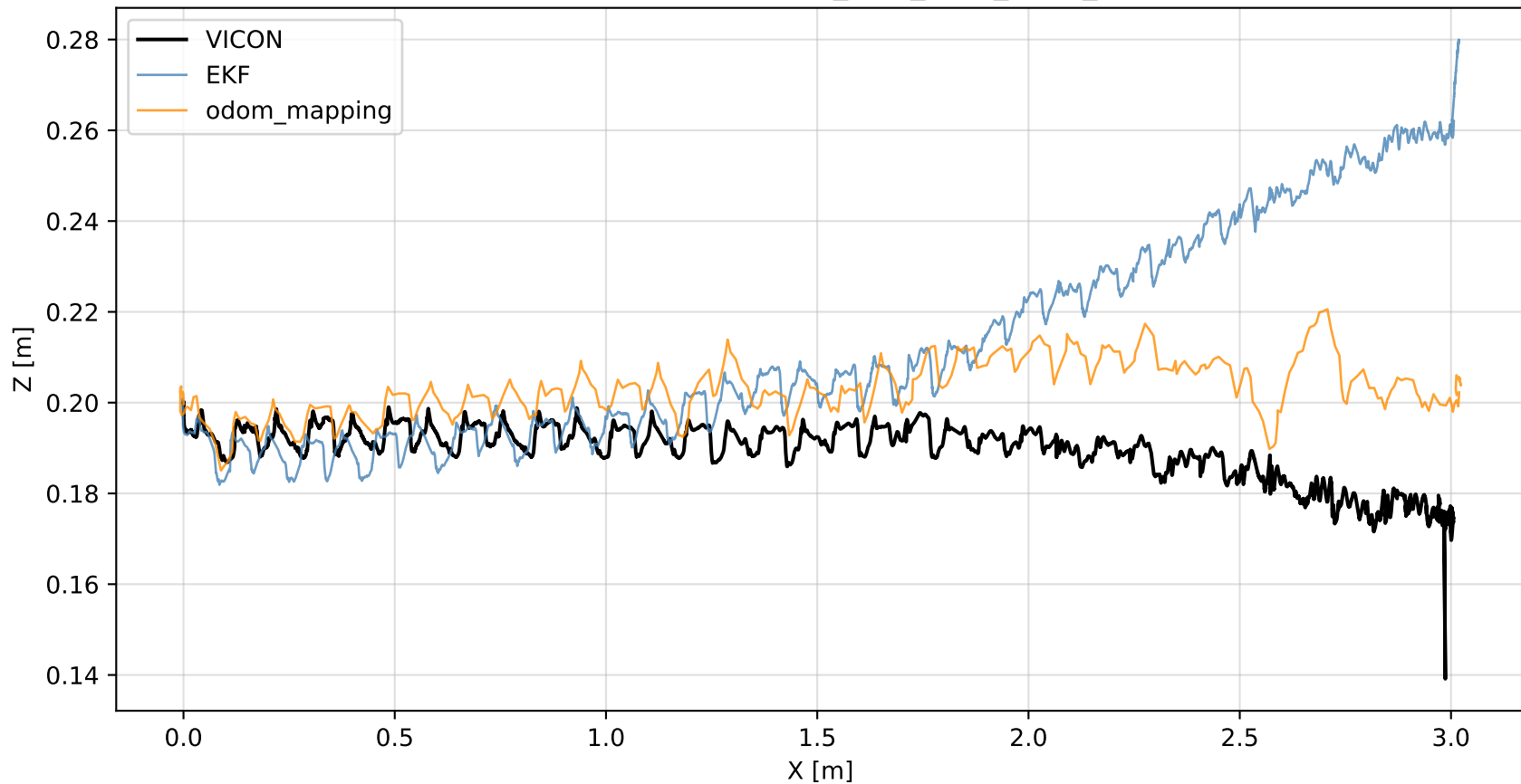
XZ Trajectory — FLAT_MPC_NEW_REAL_4
