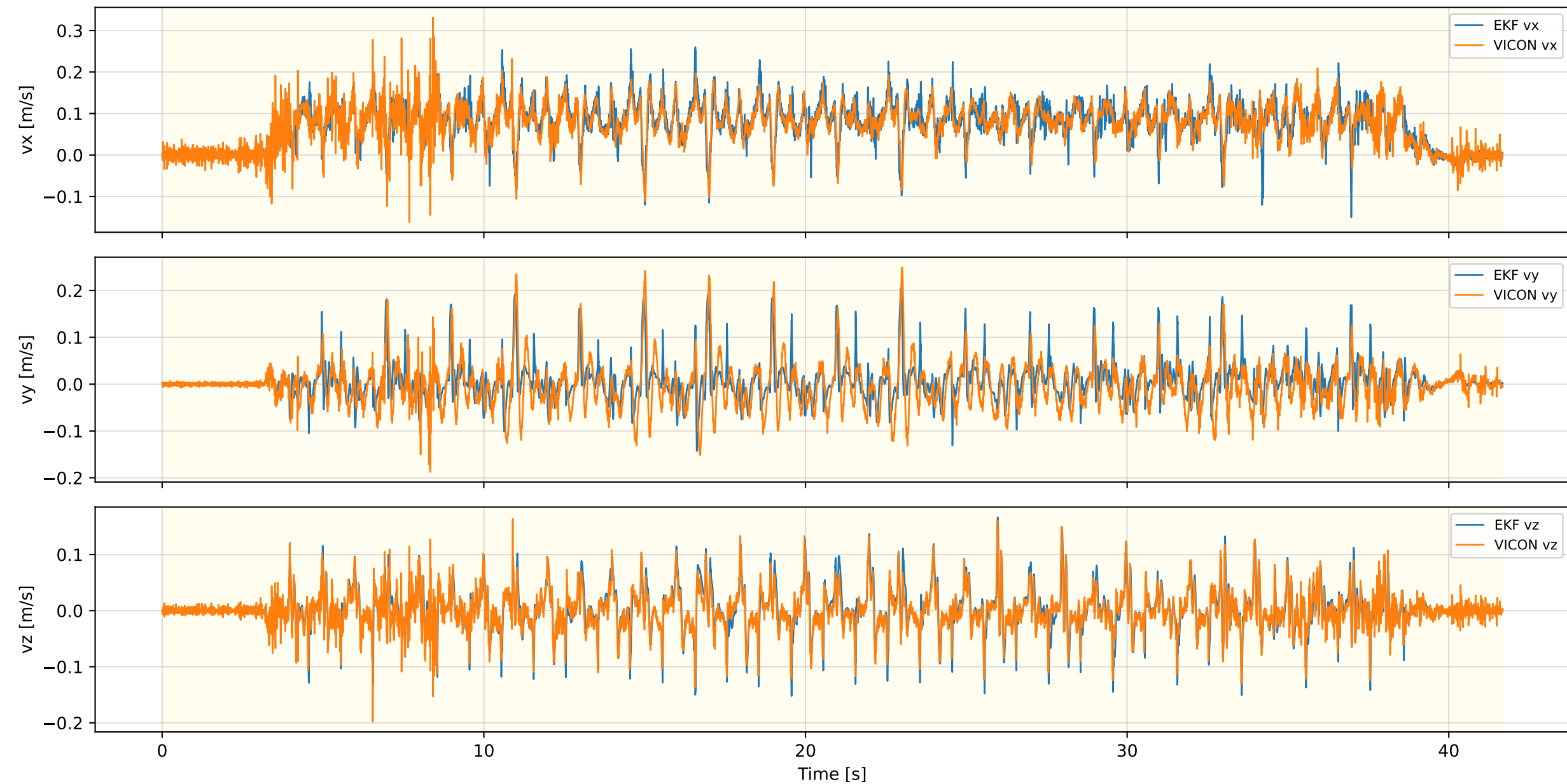
Inner EKF Velocity — FLAT_MPC_NEW_REAL_5
