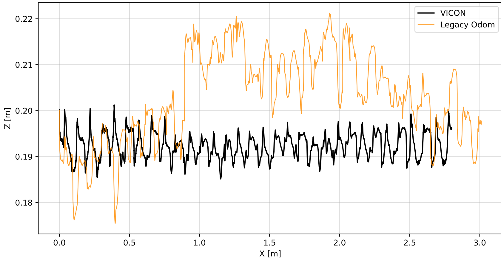
XZ Trajectory — FLAT_MPC_OLD_REAL_2
