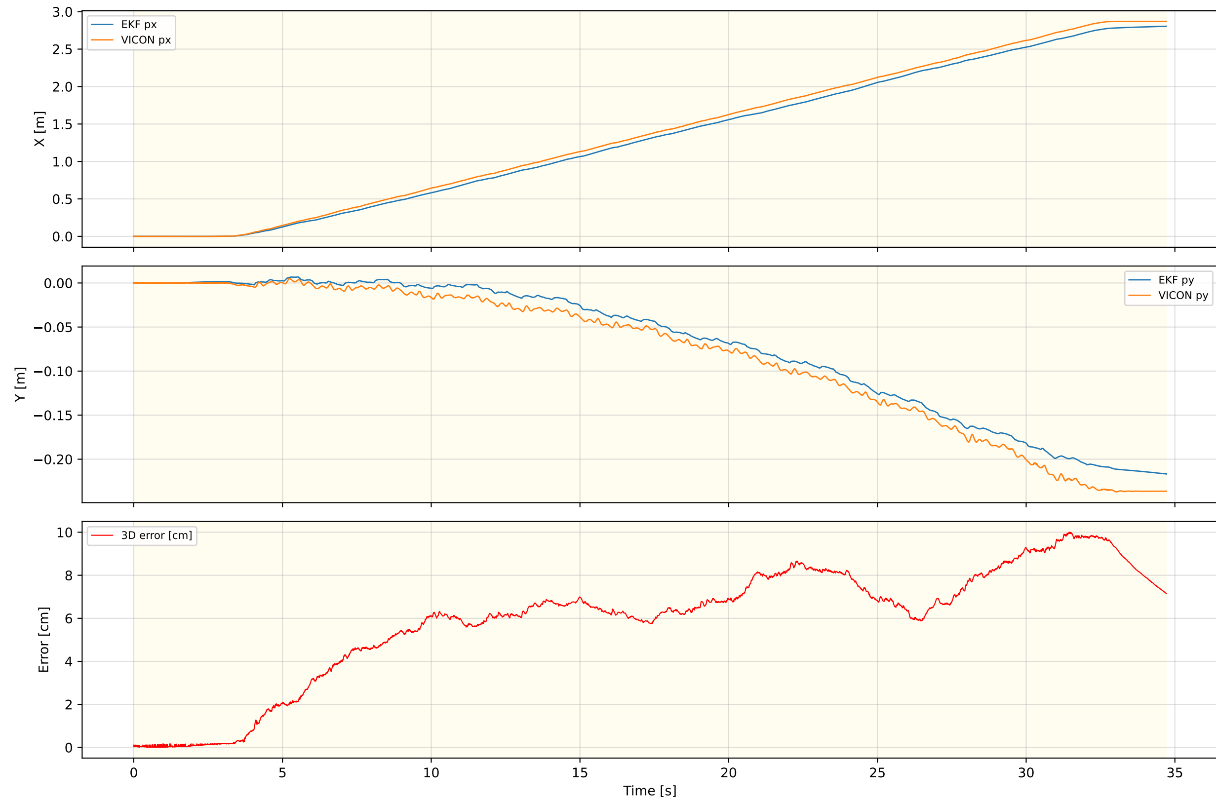
Inner EKF Position — FLAT_WLW_NEW_REAL_1
