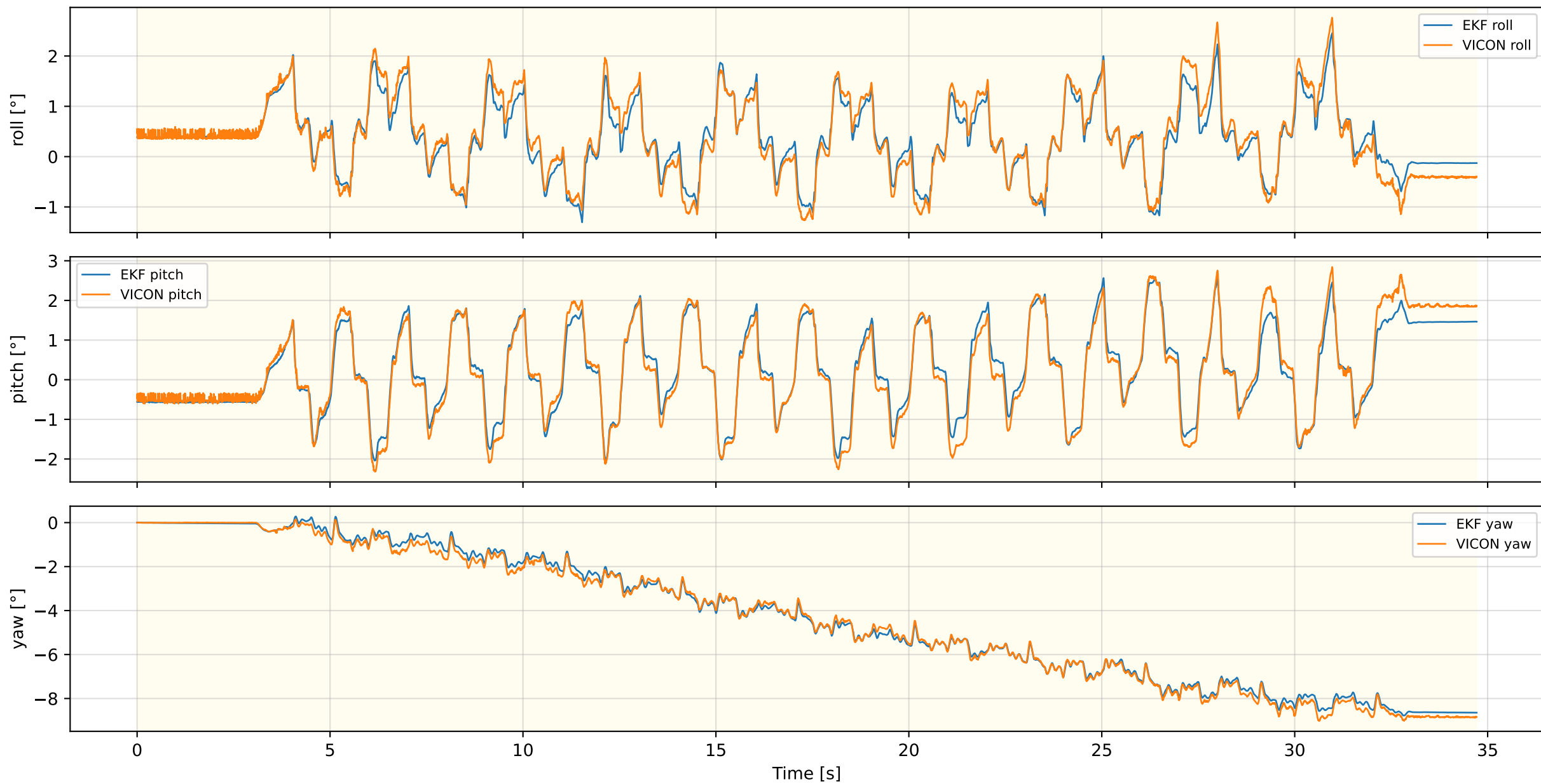
Inner EKF Attitude — FLAT_WLW_NEW_REAL_1
